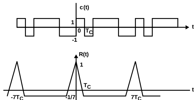
FIGURE 20. SEVEN CHIP M-SEQUENCE AND ITS AUTOCORRELATION FUNCTION
