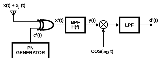
FIGURE 17. DSSS RECEIVER
