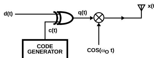
FIGURE 16. DSSS TRANSMITTER
