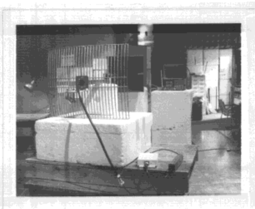
Figure 5.1, Measurement set-up in the chamber. Antenna used is to the right.
