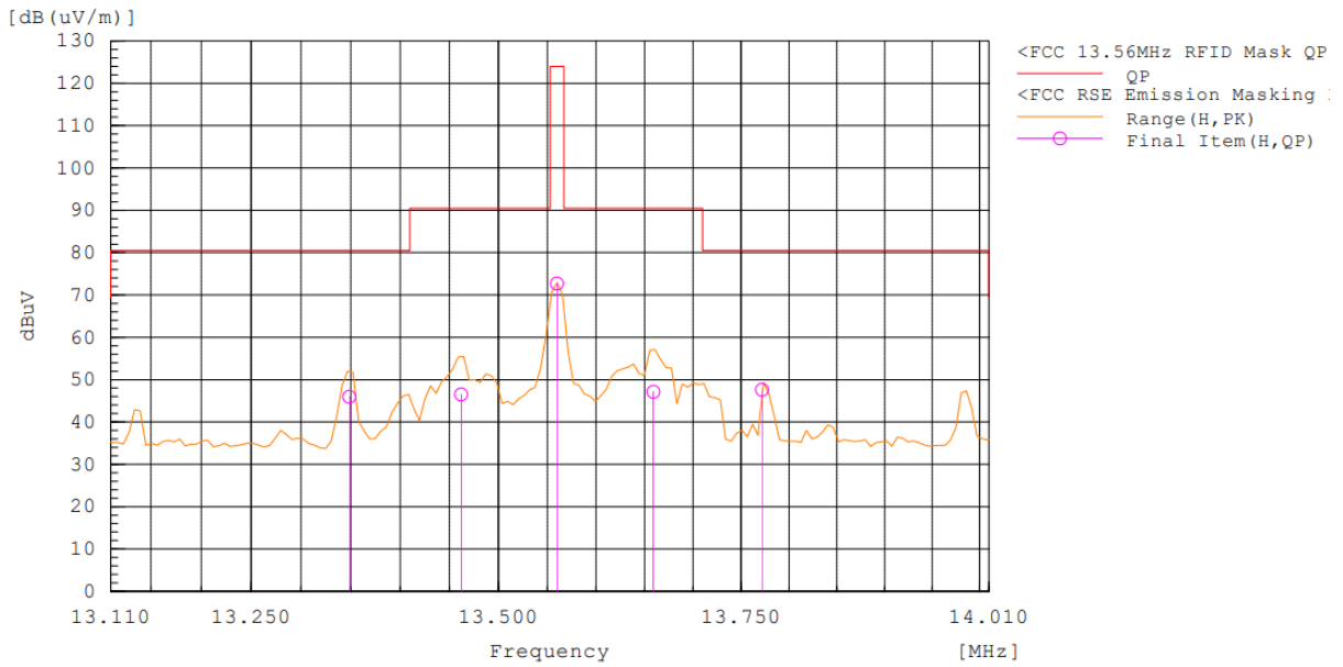
Radiated E-Field Emission (Antenna Position 90°) : 13.110 – 14.010 MHz
