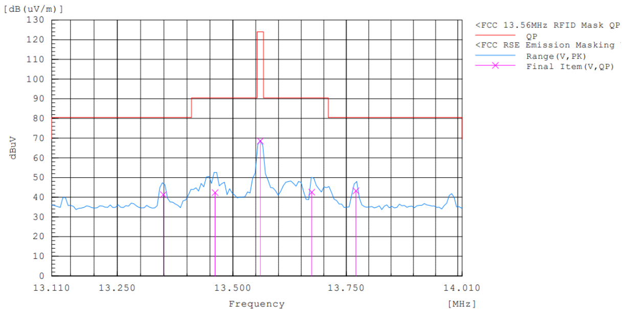
Radiated E-Field Emission (Antenna Position 90°) : 13.110 – 14.010 MHz
