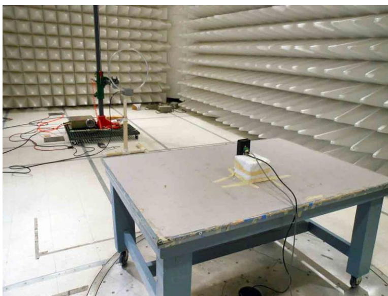
POE, 9kHz-30MHz
