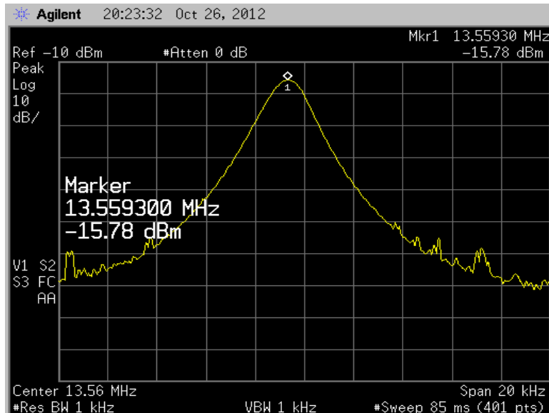
Figure 39: Carrier Frequency at 20°C for 5VDC input voltage
