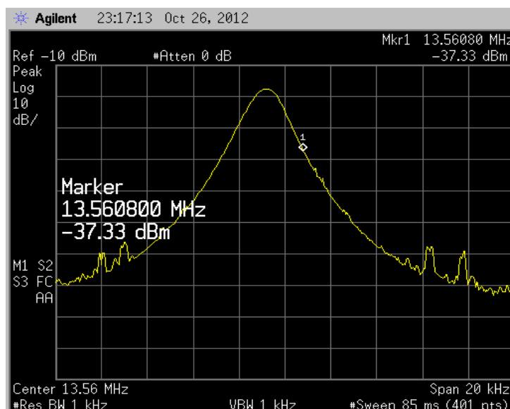
Figure 29: Measured f_H for 20dB Bandwidth
