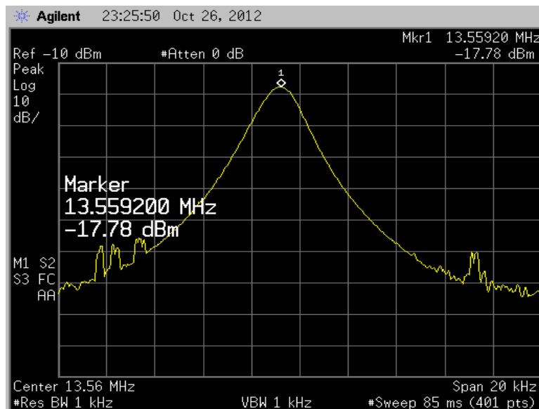
Figure 46: Carrier Frequency at 20°C for 5.75VDC input voltage
