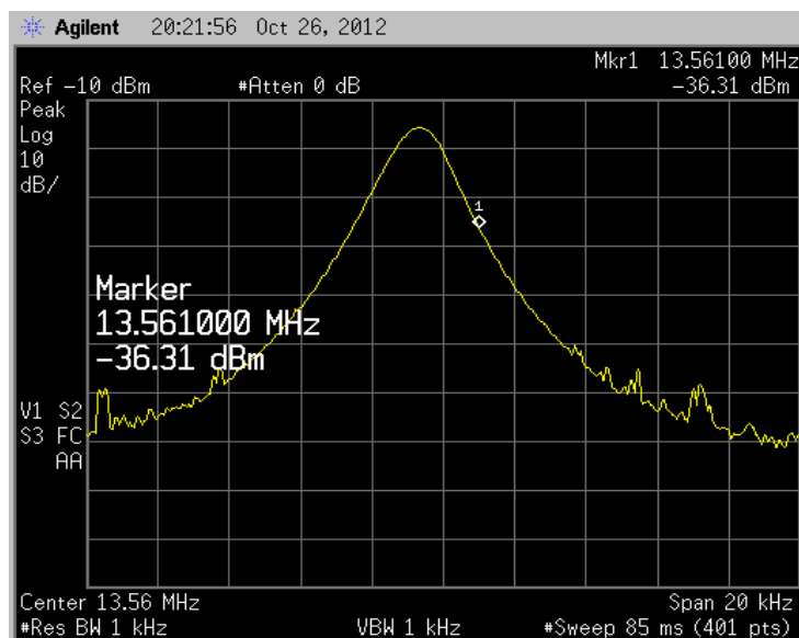
Figure 26: Measured f_H for 20dB Bandwidth
