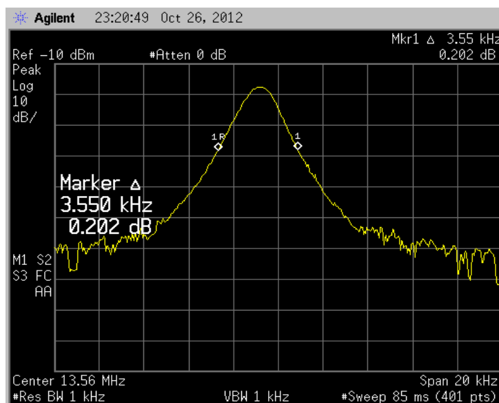
Figure 30: 20dB Bandwidth plot
