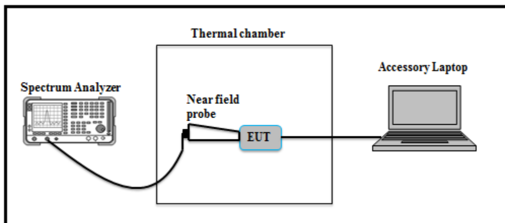
Figure 34: Sample test setup for Frequency stability measurement
