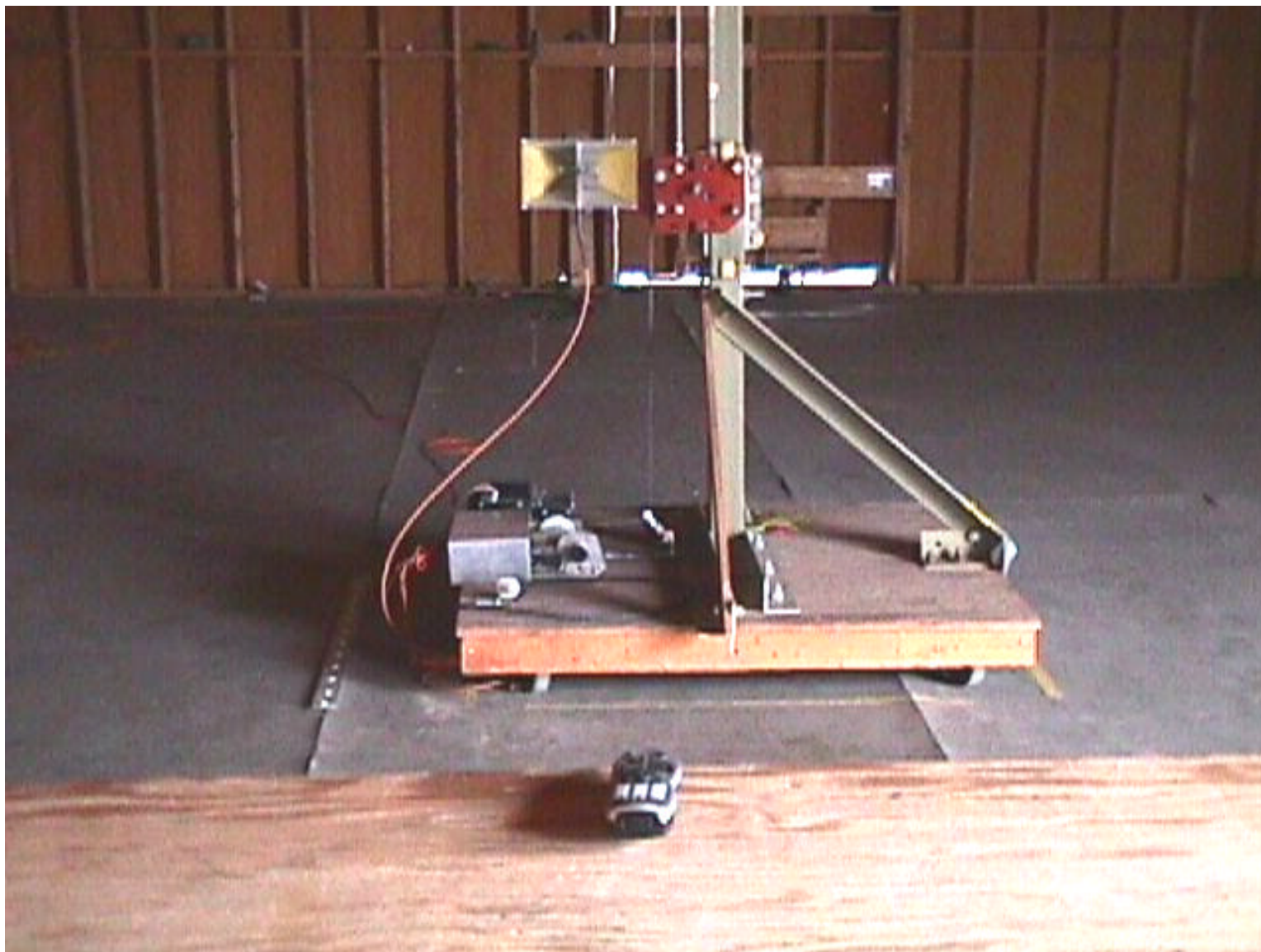
Test Setup for Radiated Emissions - Handset Unit (Orthogonal Position #2)
