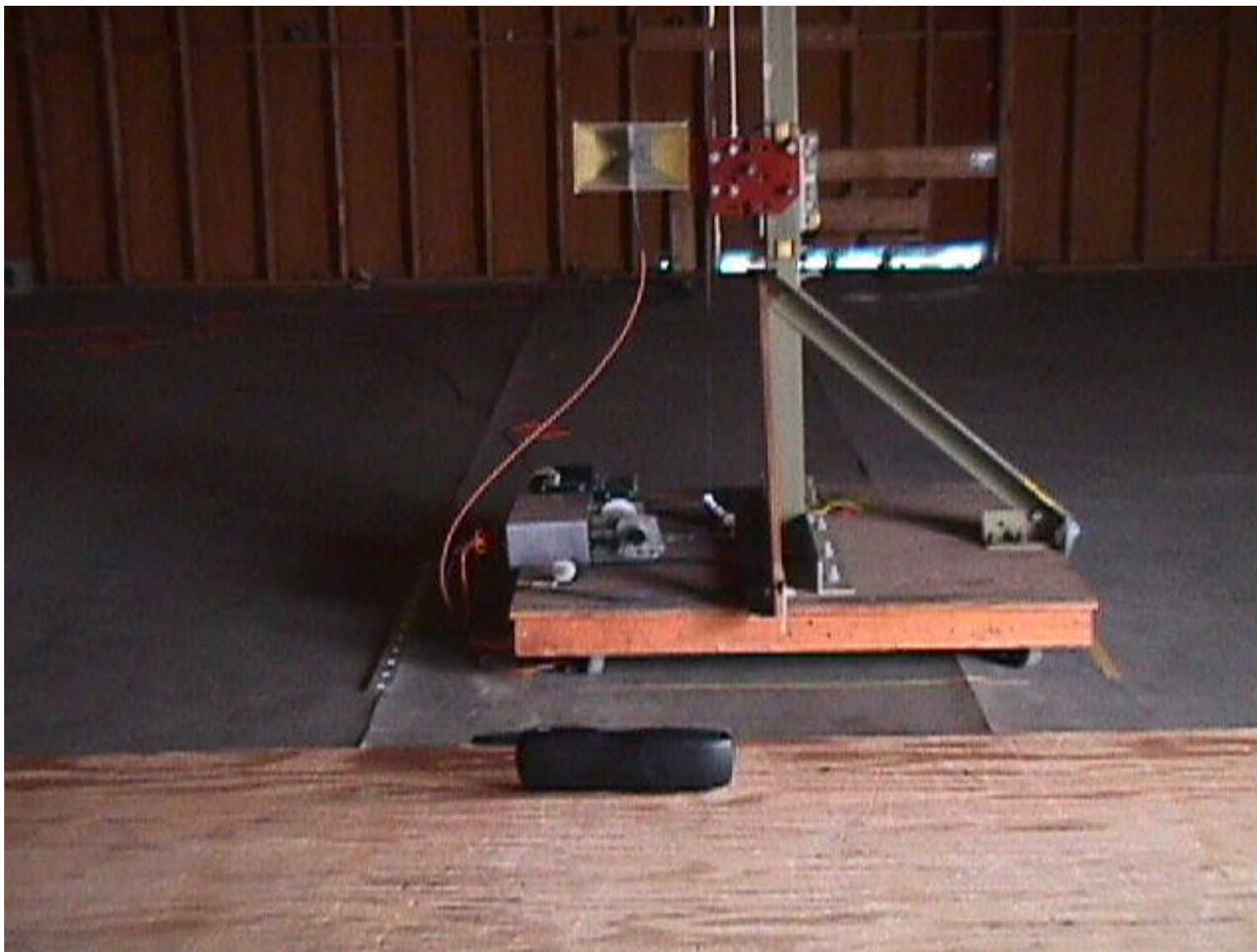
Test Setup for Radiated Emissions - Handset Unit (Orthogonal Position #1)
