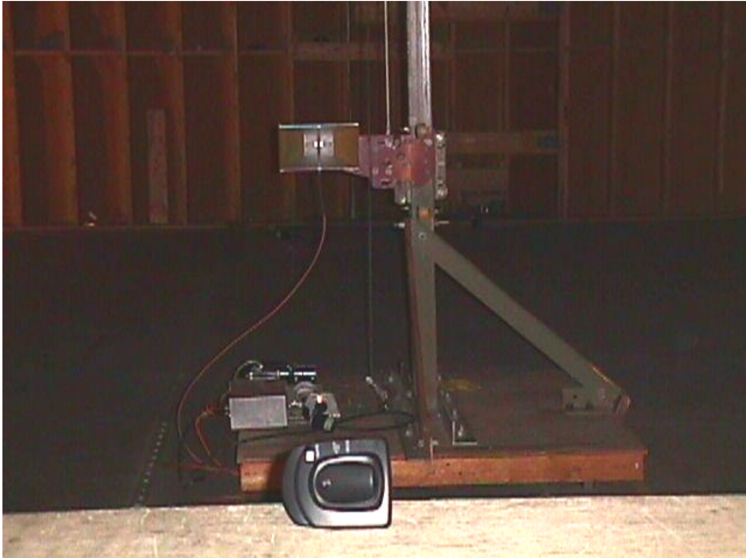
Test Setup for Radiated Emissions - Base Unit
