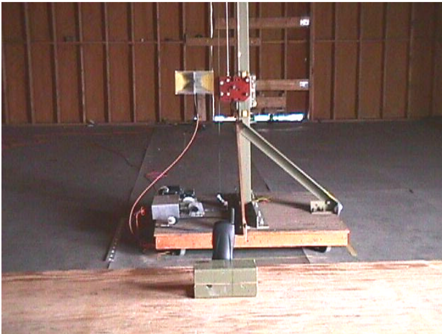
Test Setup for Radiated Emissions - Handset Unit (Orthogonal Position #3)
