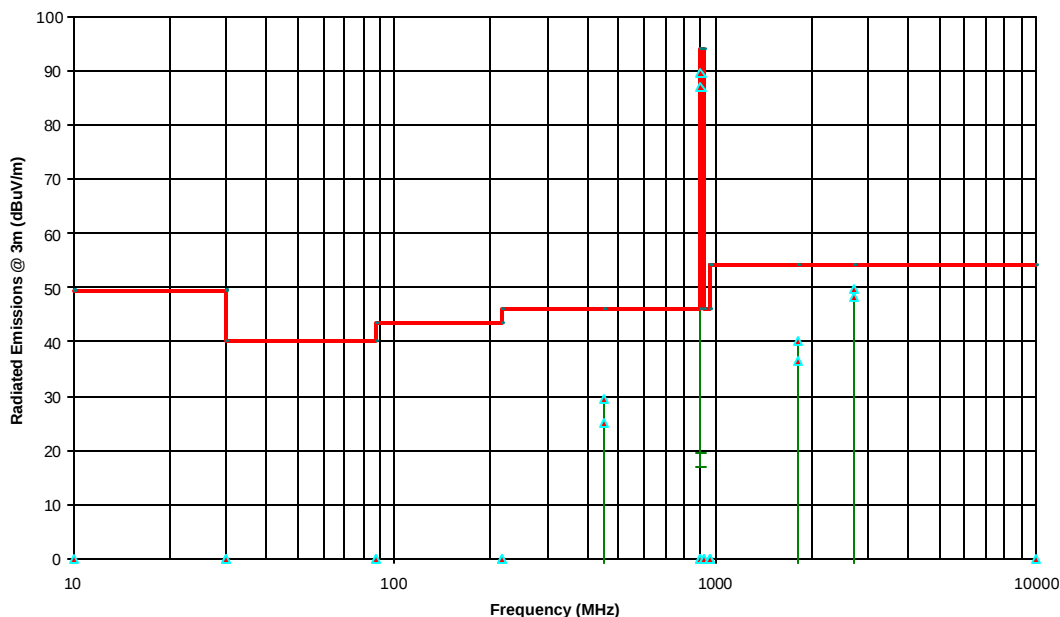
Radiated Emissions Measurements @ 3m OFTS Sanyo 900 MHz Cordless Telephone, Model CTL-9935N Base Channel Frequency @ 902.80 MHz
