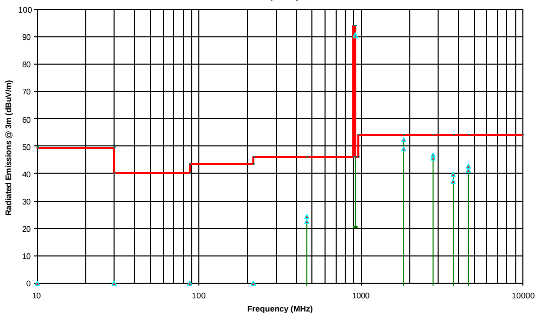
Radiated Emissions Measurements @ 3m OFTS Sanyo 900 MHz Cordless Telephone, Model CTL-9935N Handset Channel Frequency @ 925.30 MHz
