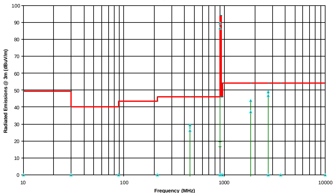
Radiated Emissions Measurements @ 3m OFTS Sanyo 900 MHz Cordless Telephone, Model CTL-9935N Base Channel Frequency @ 904.75 MHz
