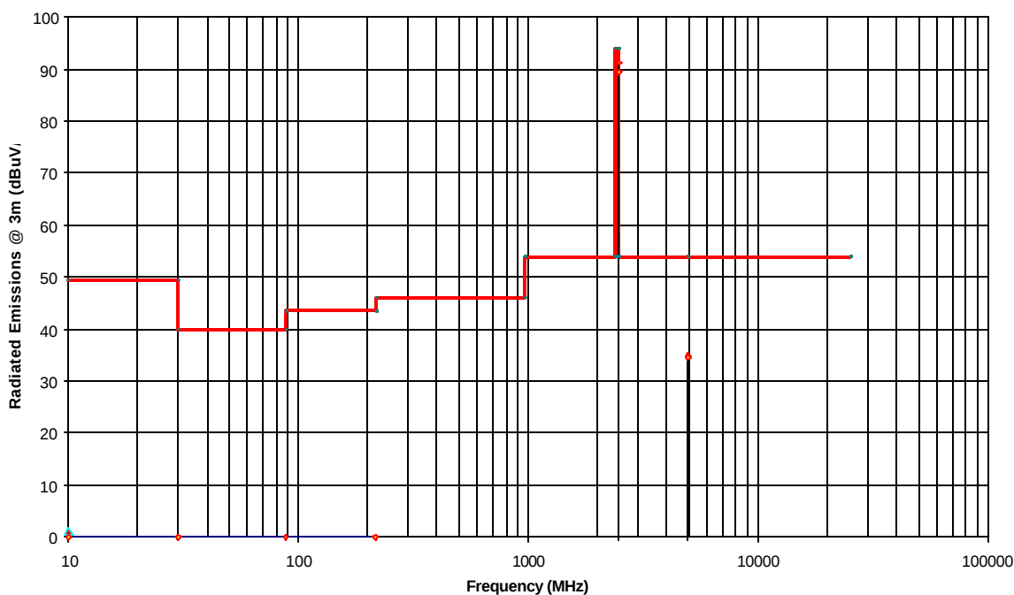
Radiated Emissions Measurements @ 3m OFTS Sanyo 2.4 GHz Cordless Telephone, Model CTL2422 Handset Channel Frequency @ 2474.249 MHz (lowest)
