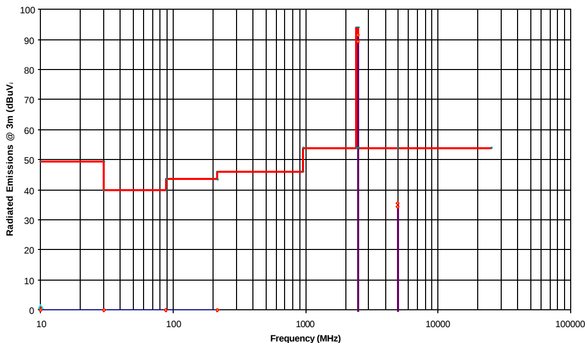
Radiated Emissions Measurements @ 3m OFTS Sanyo 2.4 GHz Cordless Telephone, Model CTL2422 Handset Channel Frequency @ 2475.199 MHz (middle)
