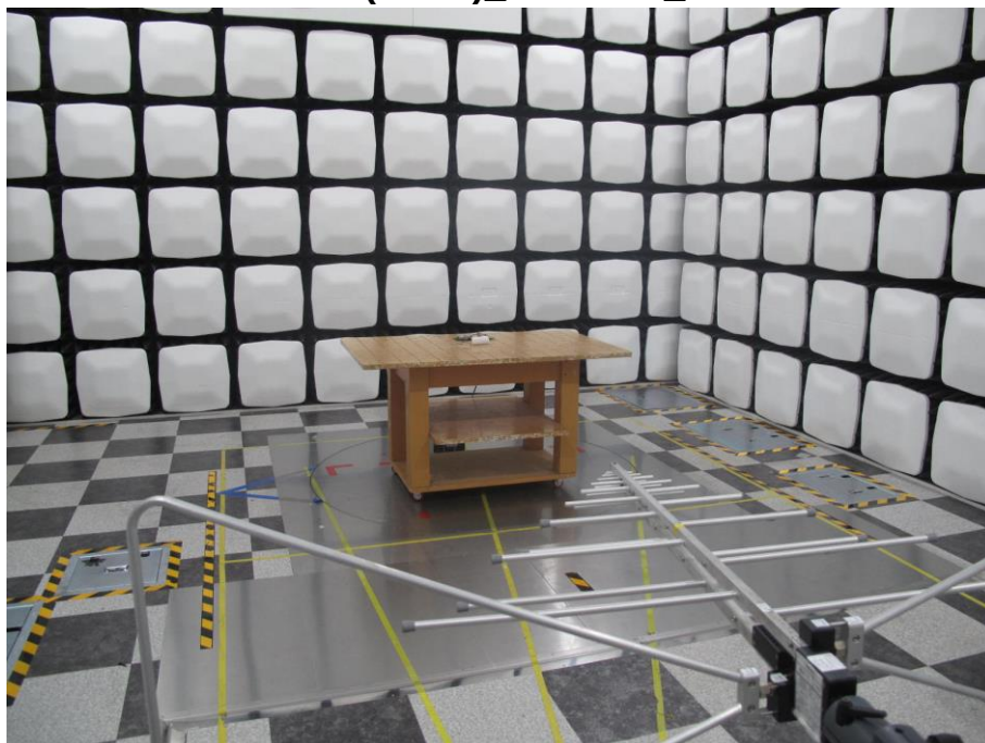
Radiated Test Picture(Front)_ PIFA Ant_Below 1GHz
