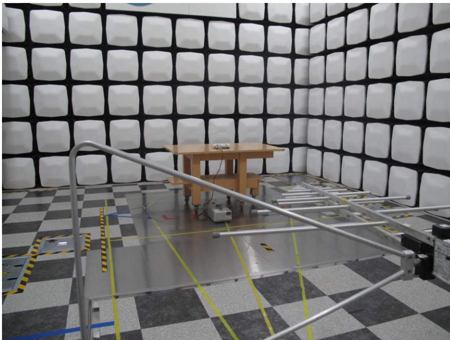
Radiated Test Picture(Rear)_ Dipole Ant_Below 1GHz
