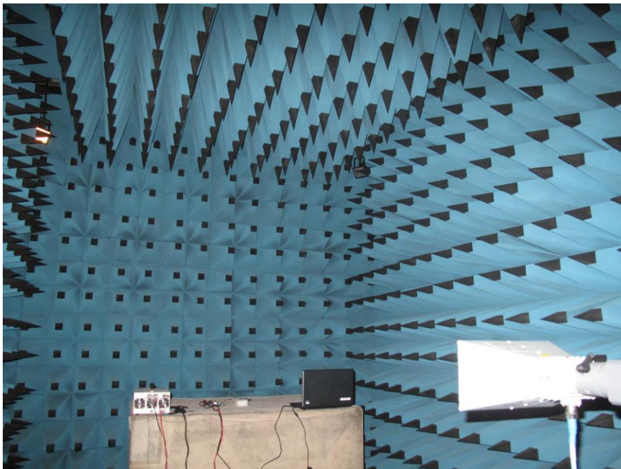
Radiated Test Picture(Rear)_ Dipole Ant_Above 1GHz
