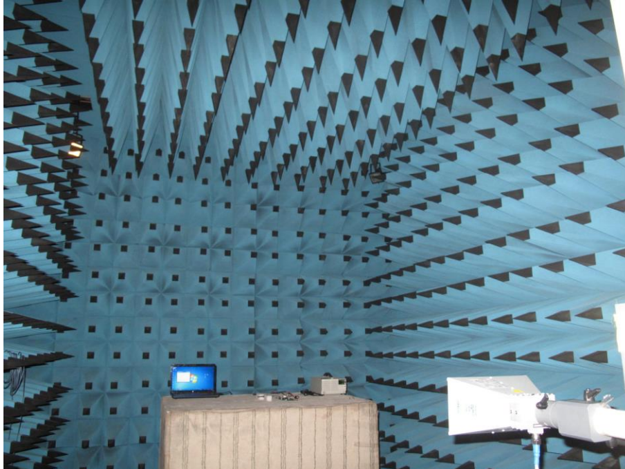
Radiated Test Picture(Front)_ Dipole Ant_Above 1GHz
