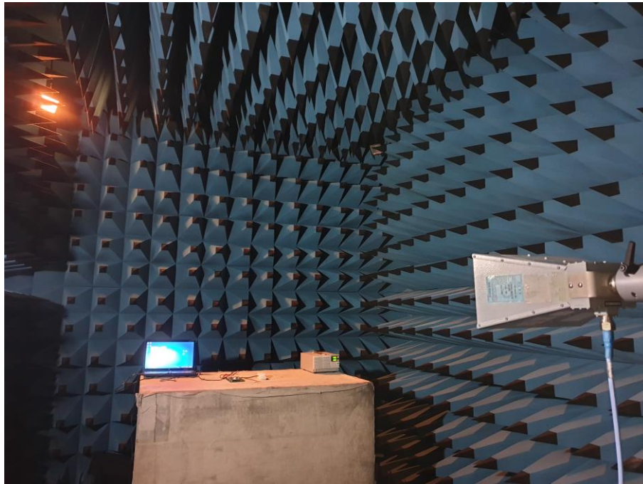
Radiated Test Picture(Front)_ PIFA Ant_Above 1GHz
