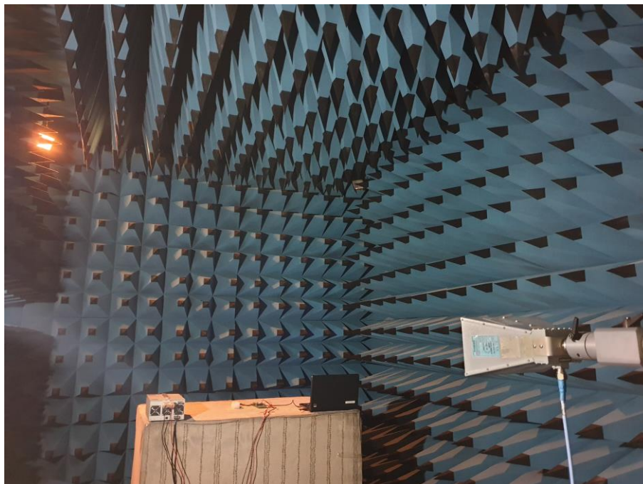
Radiated Test Picture(Rear)_ PIFA Ant_Above 1GHz
