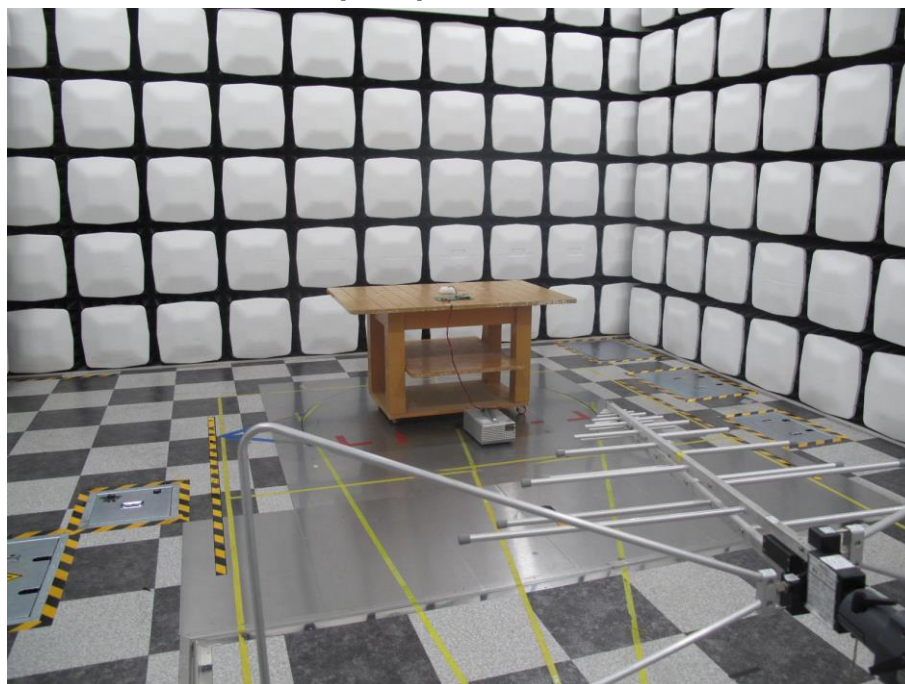
Radiated Test Picture(Rear)_ PIFA Ant_Below 1GHz
