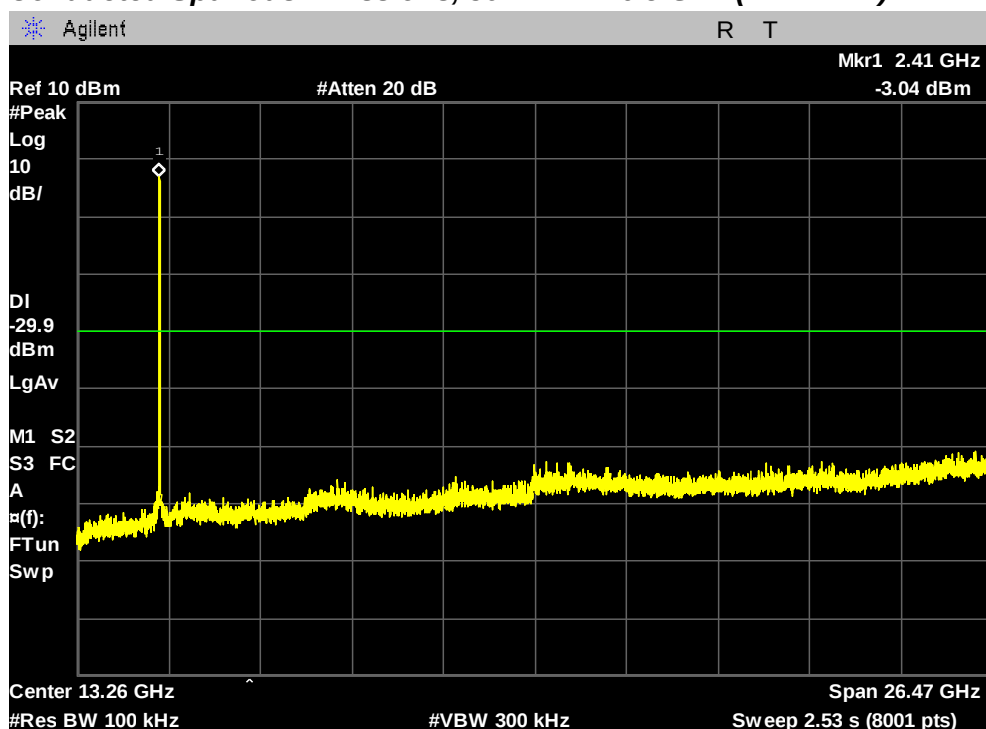
Conducted Spurious Emissions, 30 MHz ~ 26.5 GHz (2412 MHz)
