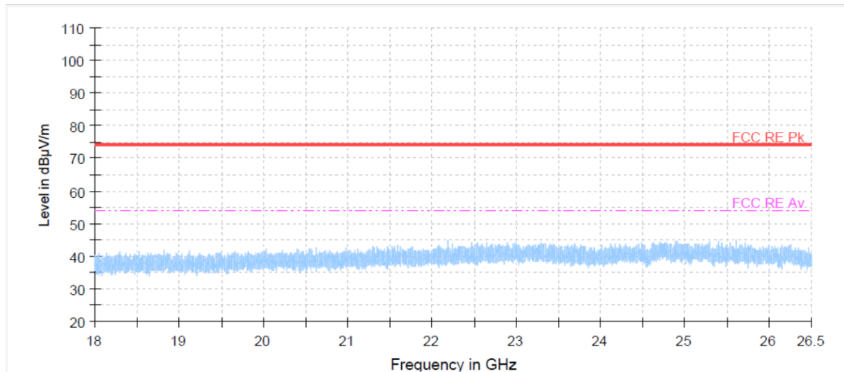
11 channel : 18 GHz to 26.5 GHz_Peak
