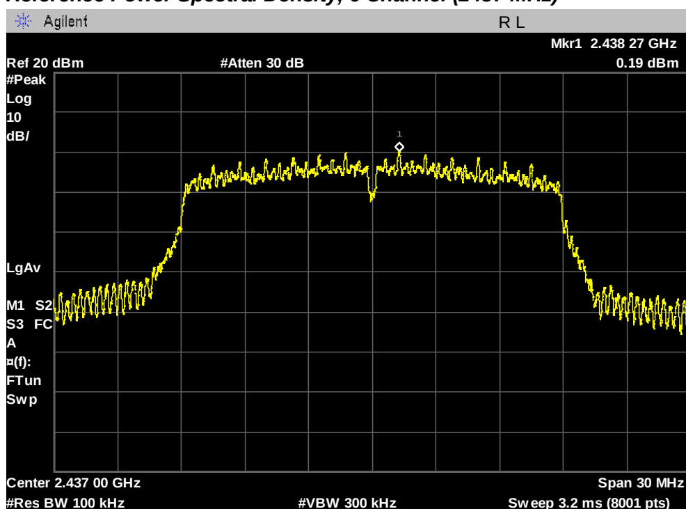
Reference Power Spectral Density, 6 Channel (2437 MHz)
