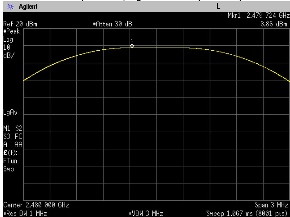
Maximum Peak Output Power, Highest Channel (2480 MHz)
