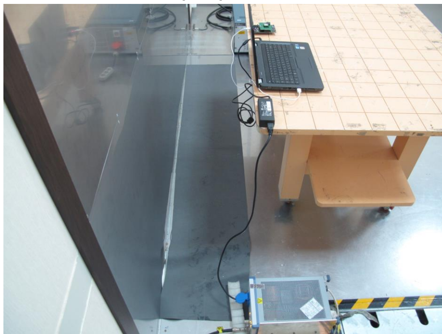
Conducted Test Picture(Rear)
