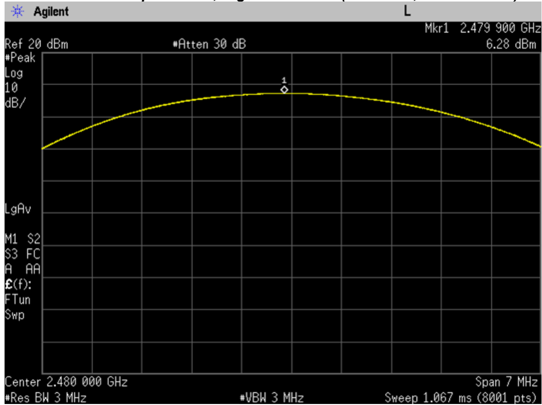
Maximum Peak Output Power, Highest channel (2480 MHz, 8DPSK Mode)
