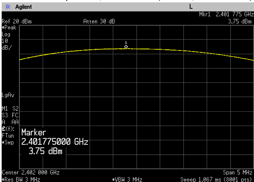
Maximum Peak Output Power, Lowest channel (2402 MHz, \pi/4 DQPSK Mode)
