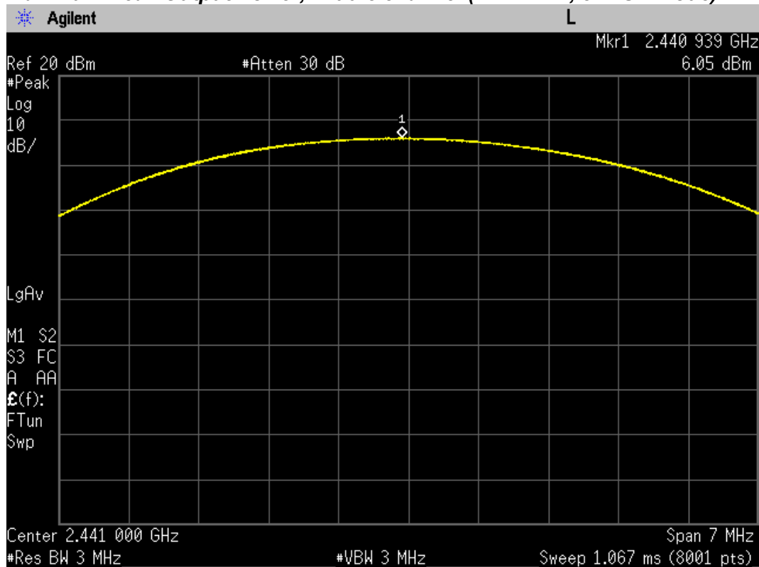
Maximum Peak Output Power, Middle channel (2441 MHz, 8DPSK Mode)
