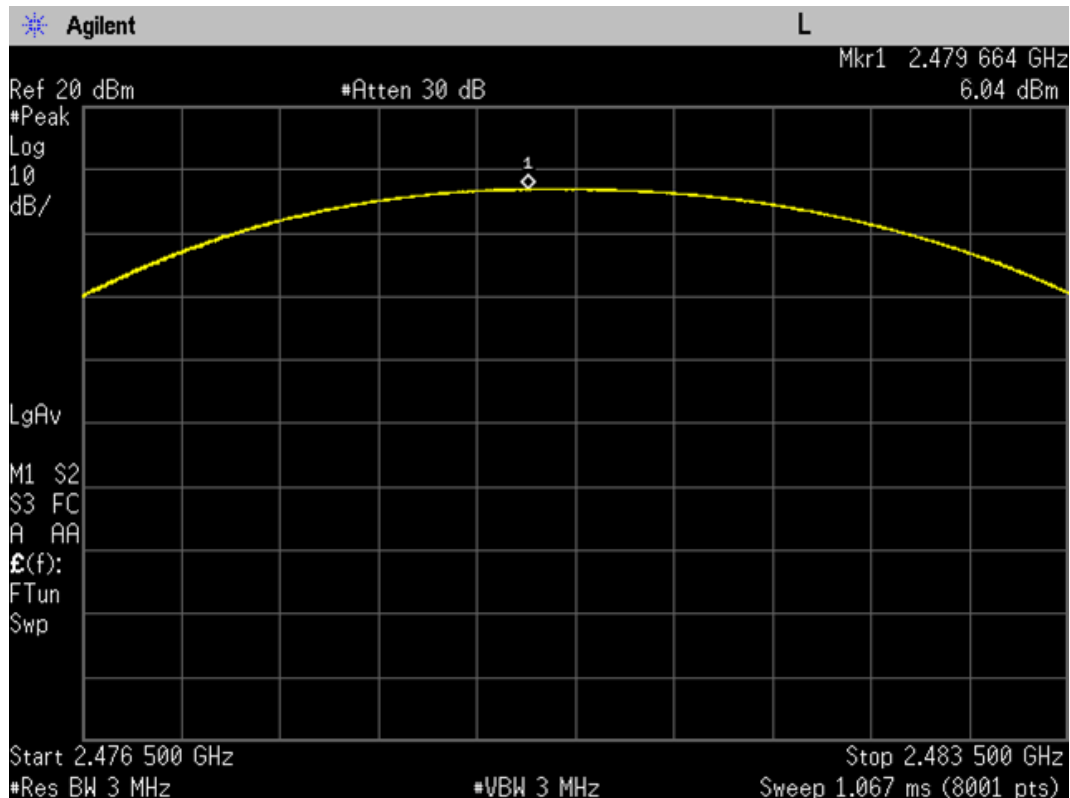
Maximum Peak Output Power, Highest channel (2480 MHz, \pi/4 DQPSK Mode)
