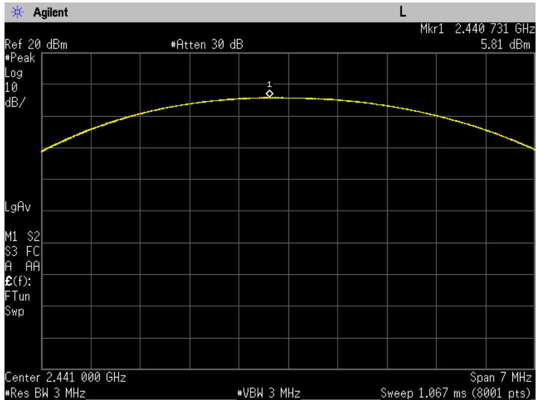
Maximum Peak Output Power, Middle channel (2441 MHz, \pi/4 DQPSK Mode)
