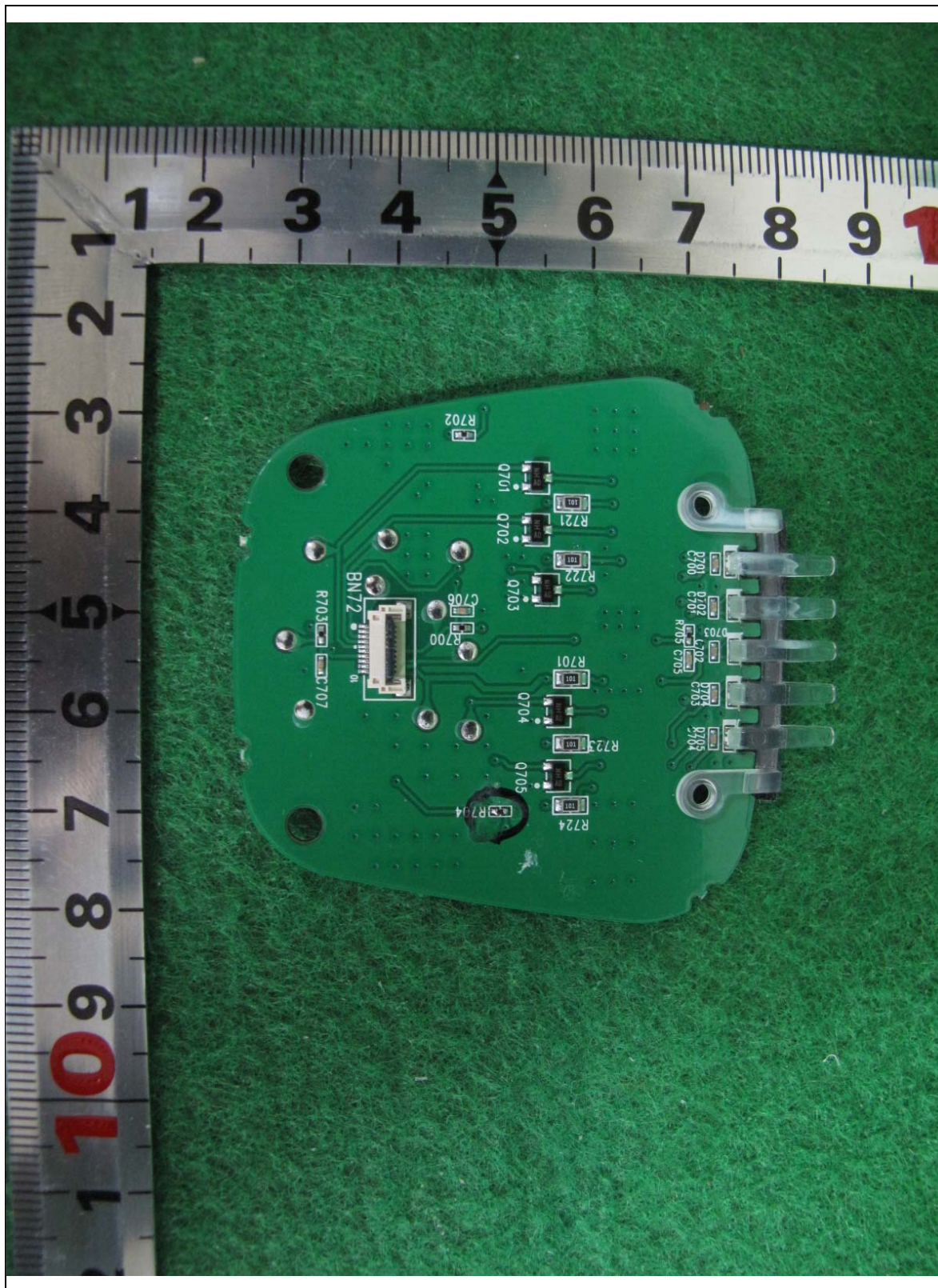
Rear View of KEY PCB
