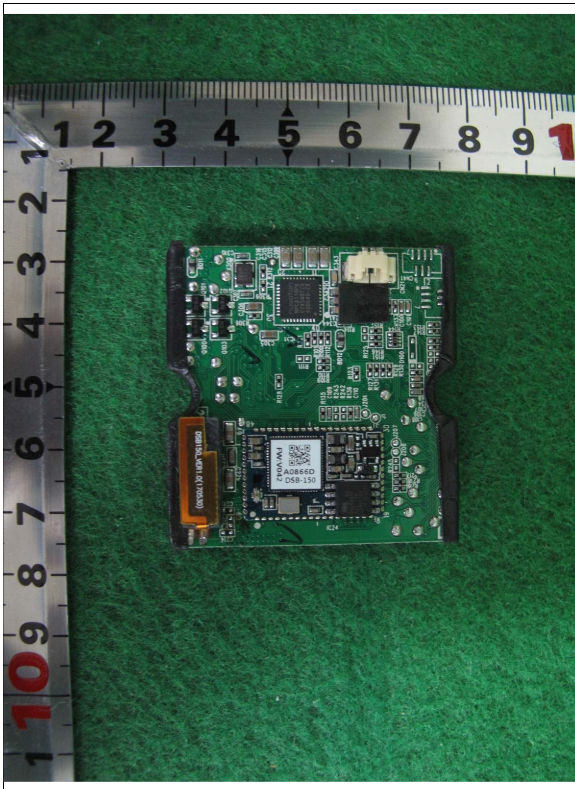
Front View of BT Module
