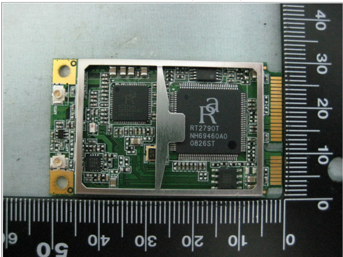
Front View of EUT-2 (AW-NE766)
