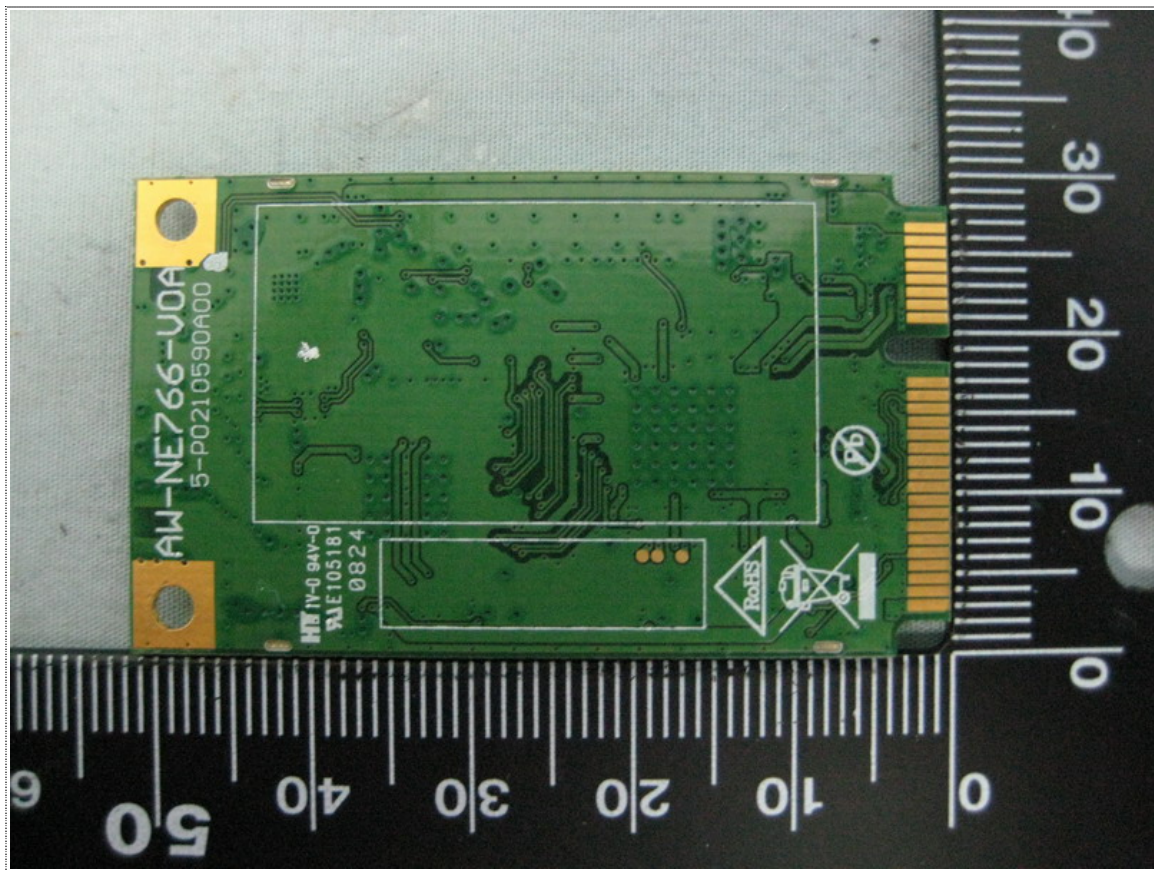
Rear View of EUT (AW-NE776)
