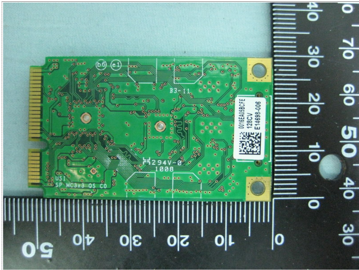
Rear View of EUT (533AN MMW)
