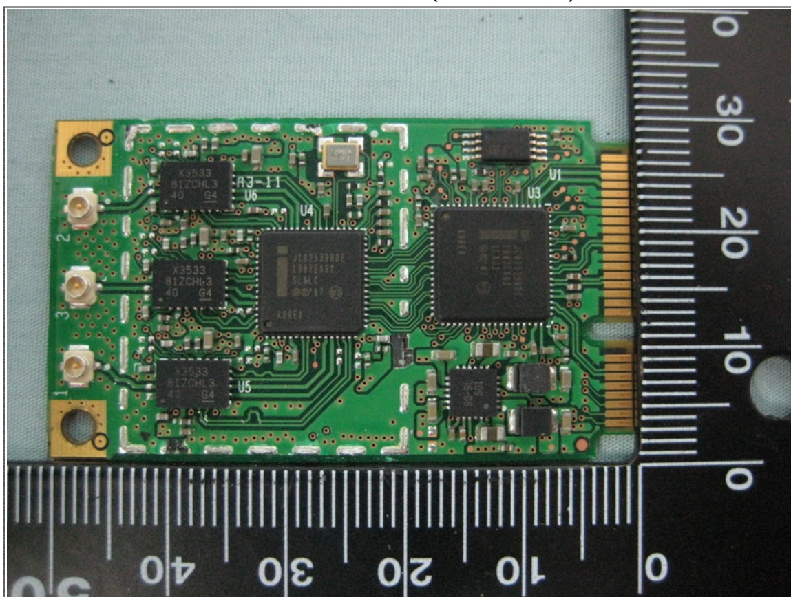
Front View of EUT-2 (533AN MMW)
