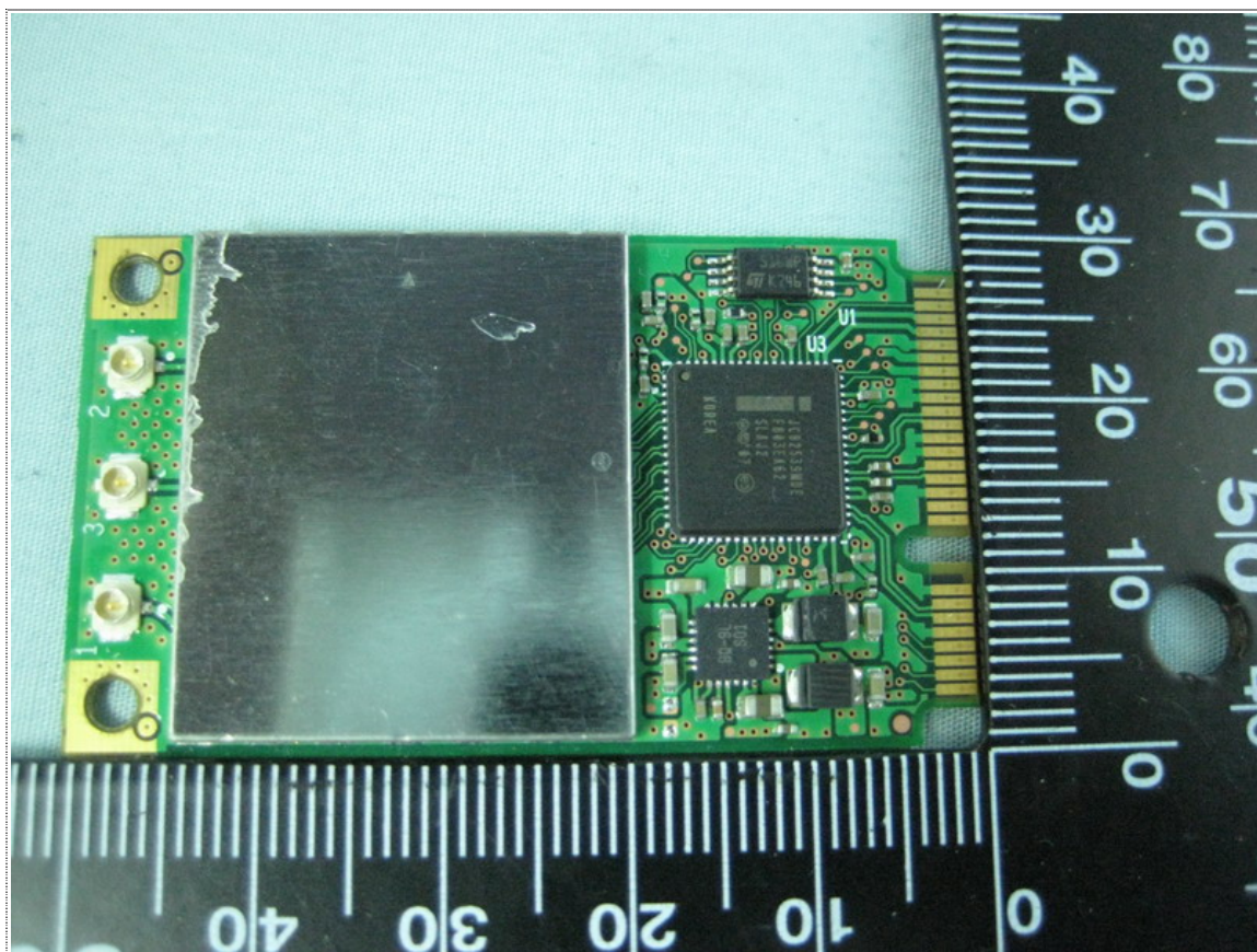
Front View of EUT-1 (533AN MMW)
