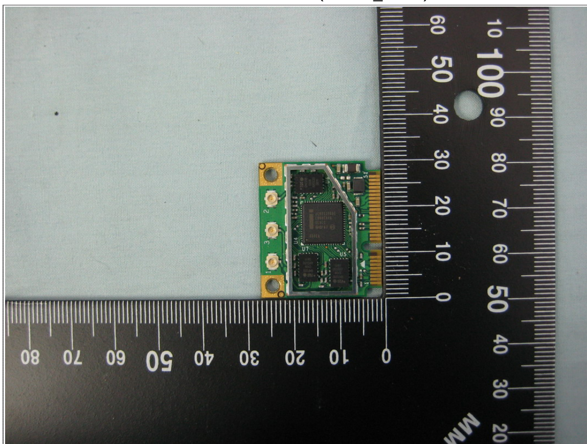
Front View of EUT-2 (533AN_HMW)
