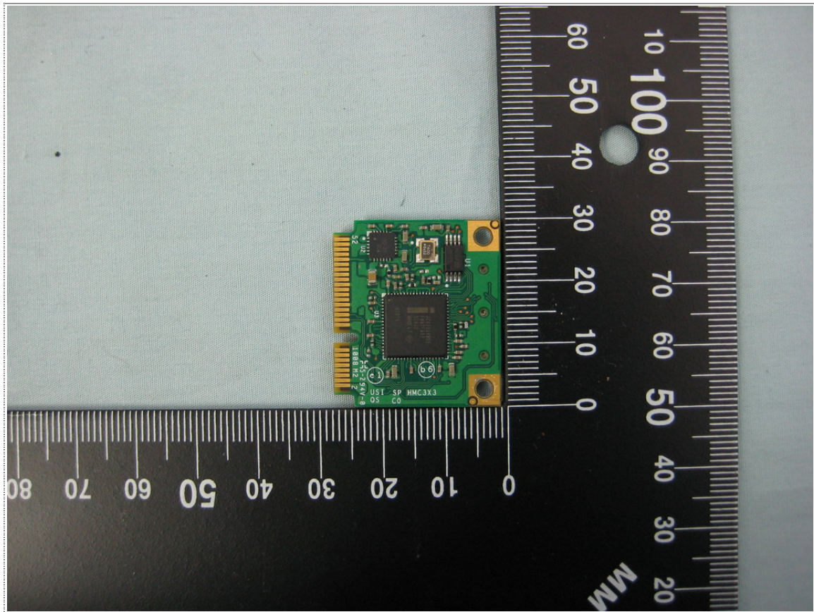
Rear View of EUT (533AN_HMW)
