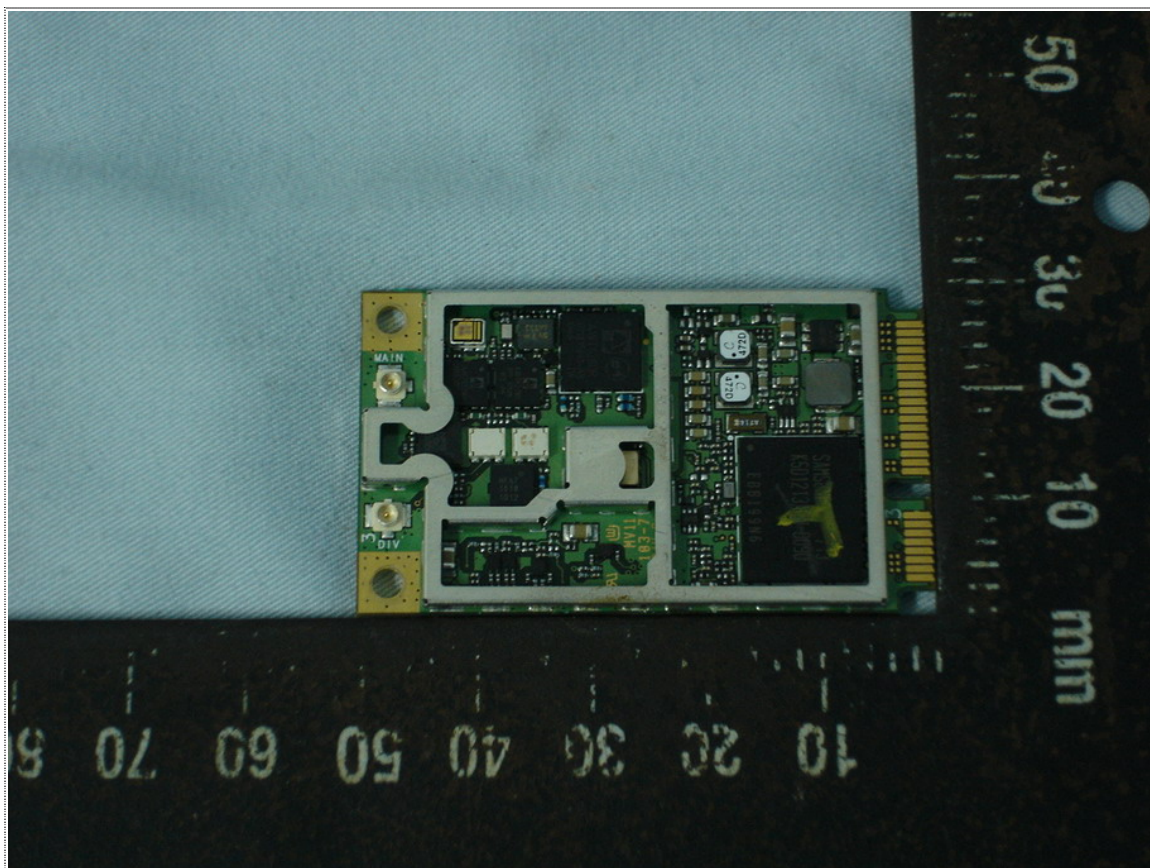
Front View of EUT-2 (EU870D)
