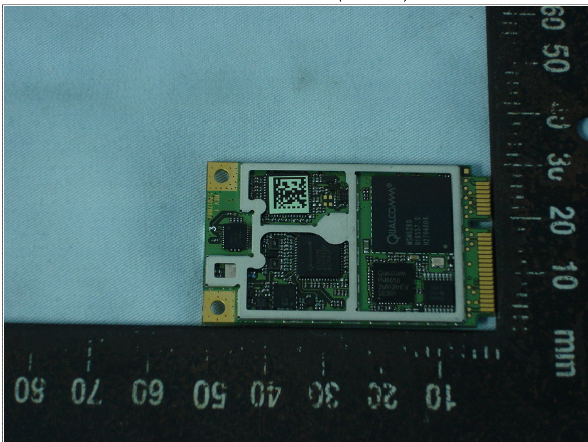
Rear View of EUT-2 (EU870D)
