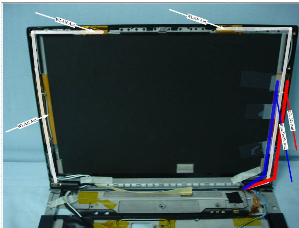
Antenna Location
