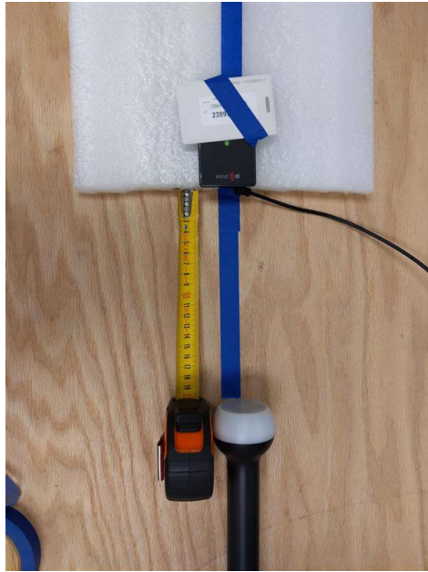
TAG ON (OFFSET) BOTTOM
