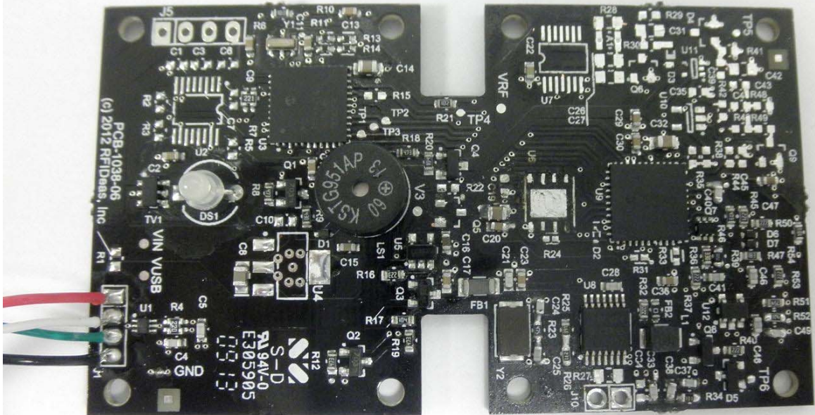
13.56MHz Mifare USB motherboard top view
