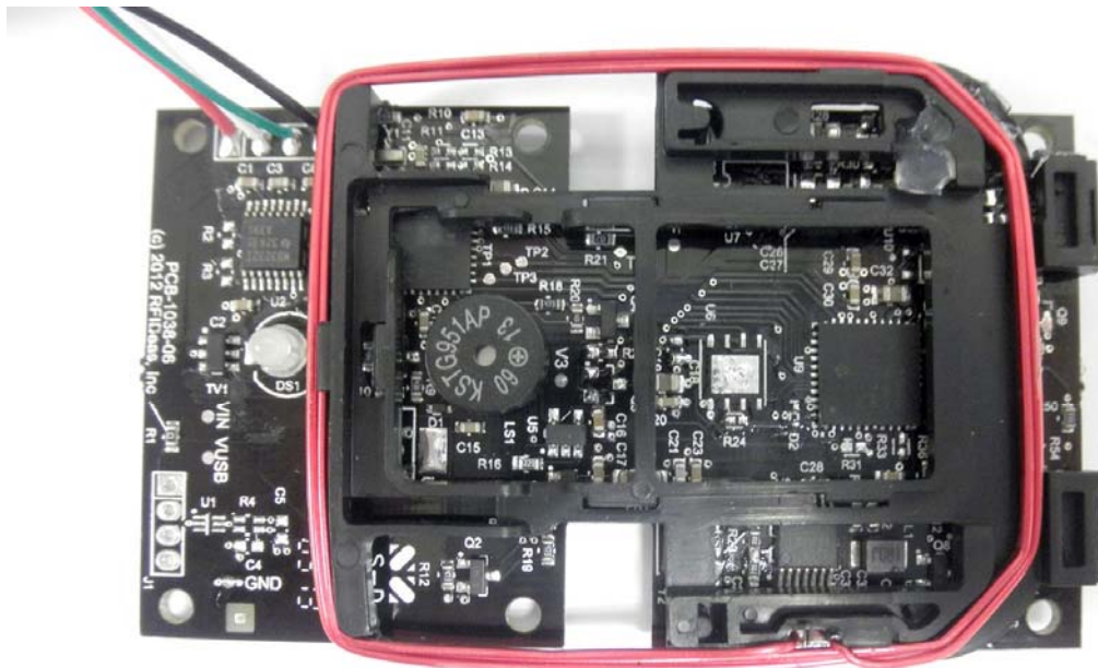
13.56MHz Mifare serial motherboard assembly top view
