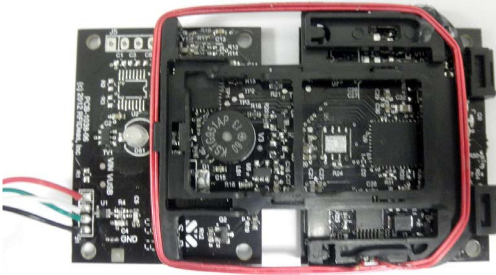
13.56MHz Mifare USB motherboard assembly top view
