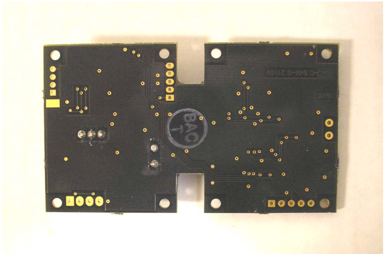
Photograph of Foil Side of PCB
