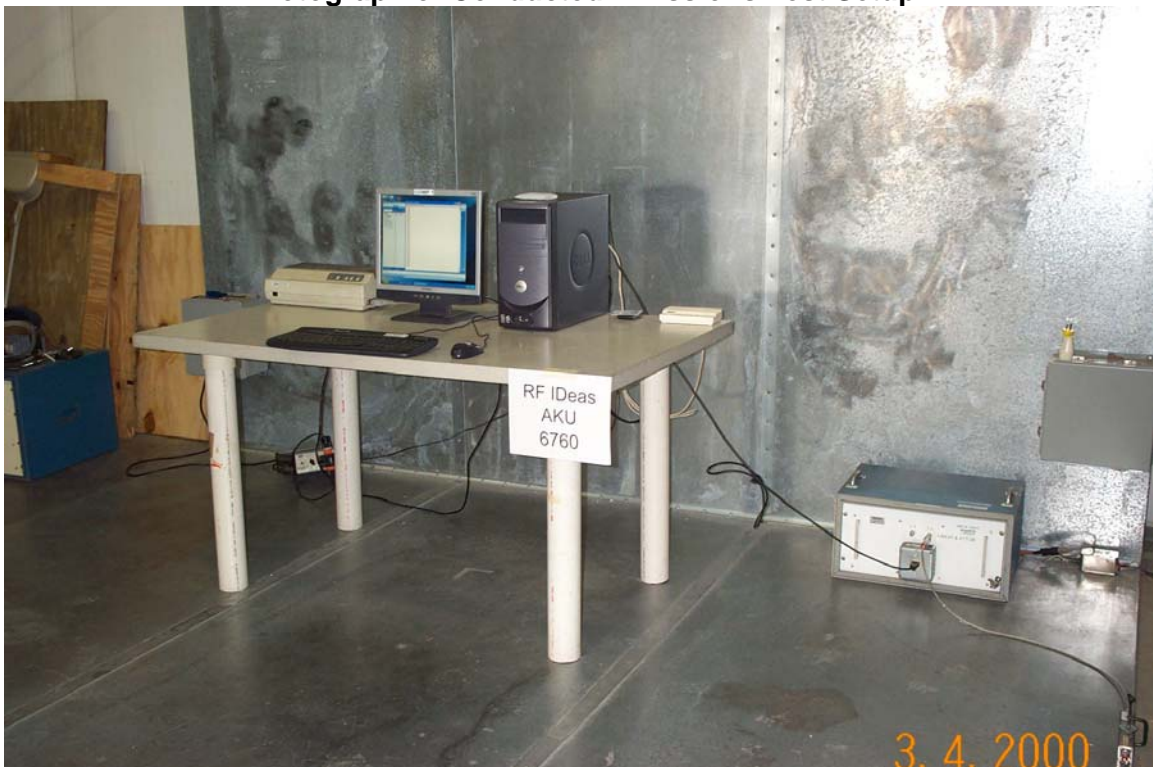
Photograph of Conducted Emissions Test Setup
