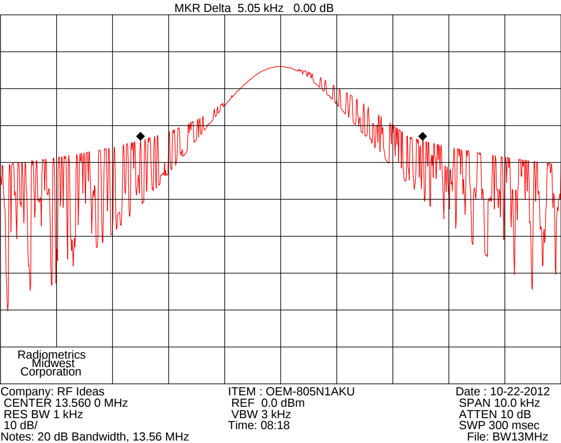
Figure 5. Occupied Bandwidth Plots 13.56 MHz
