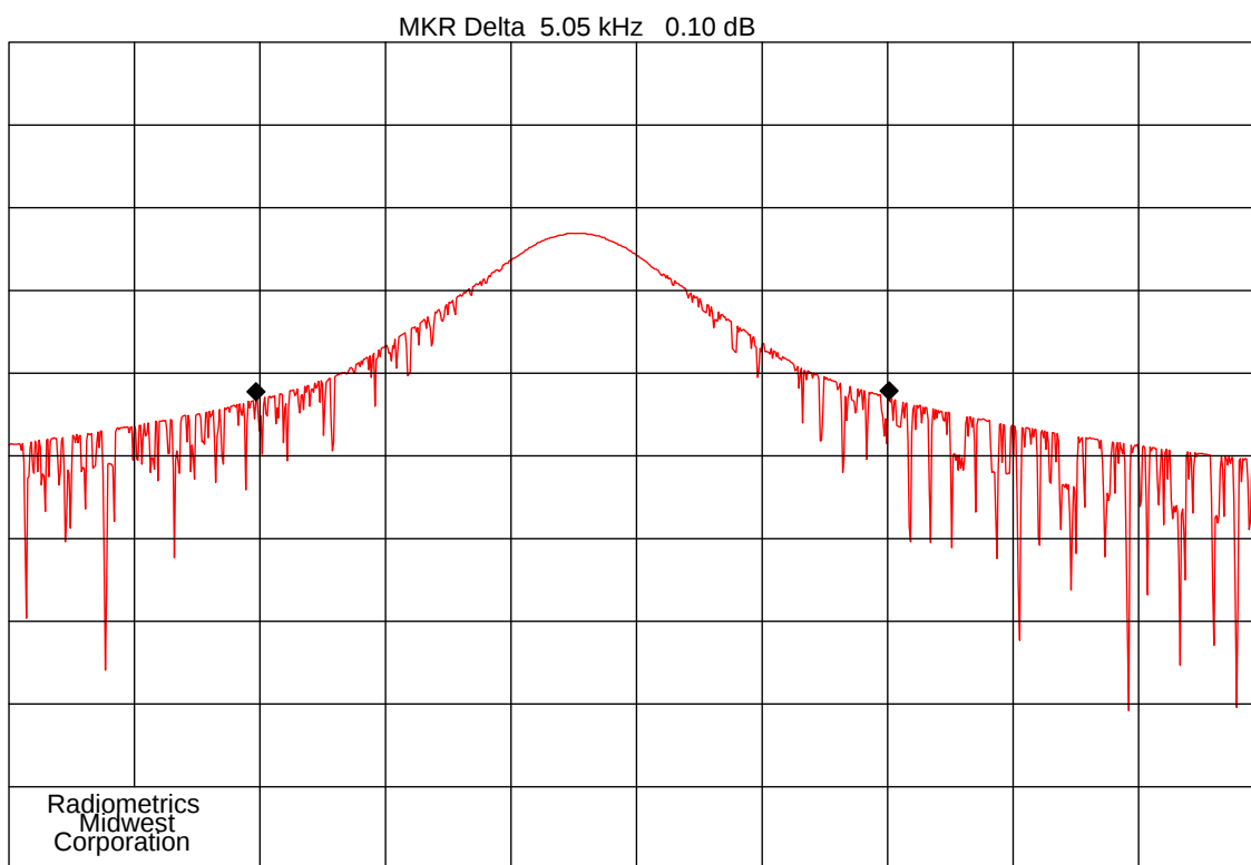
Figure 4. Occupied Bandwidth Plots 125 kHz
