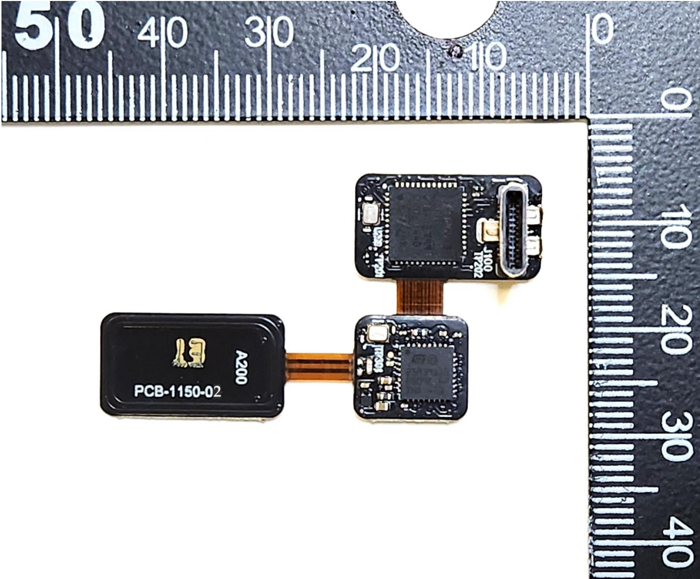
PCB's for NC-M7XC: Front
