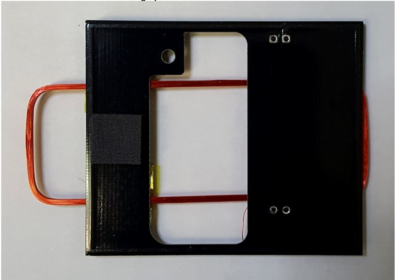
Photograph of Antenna Board: Foil side
