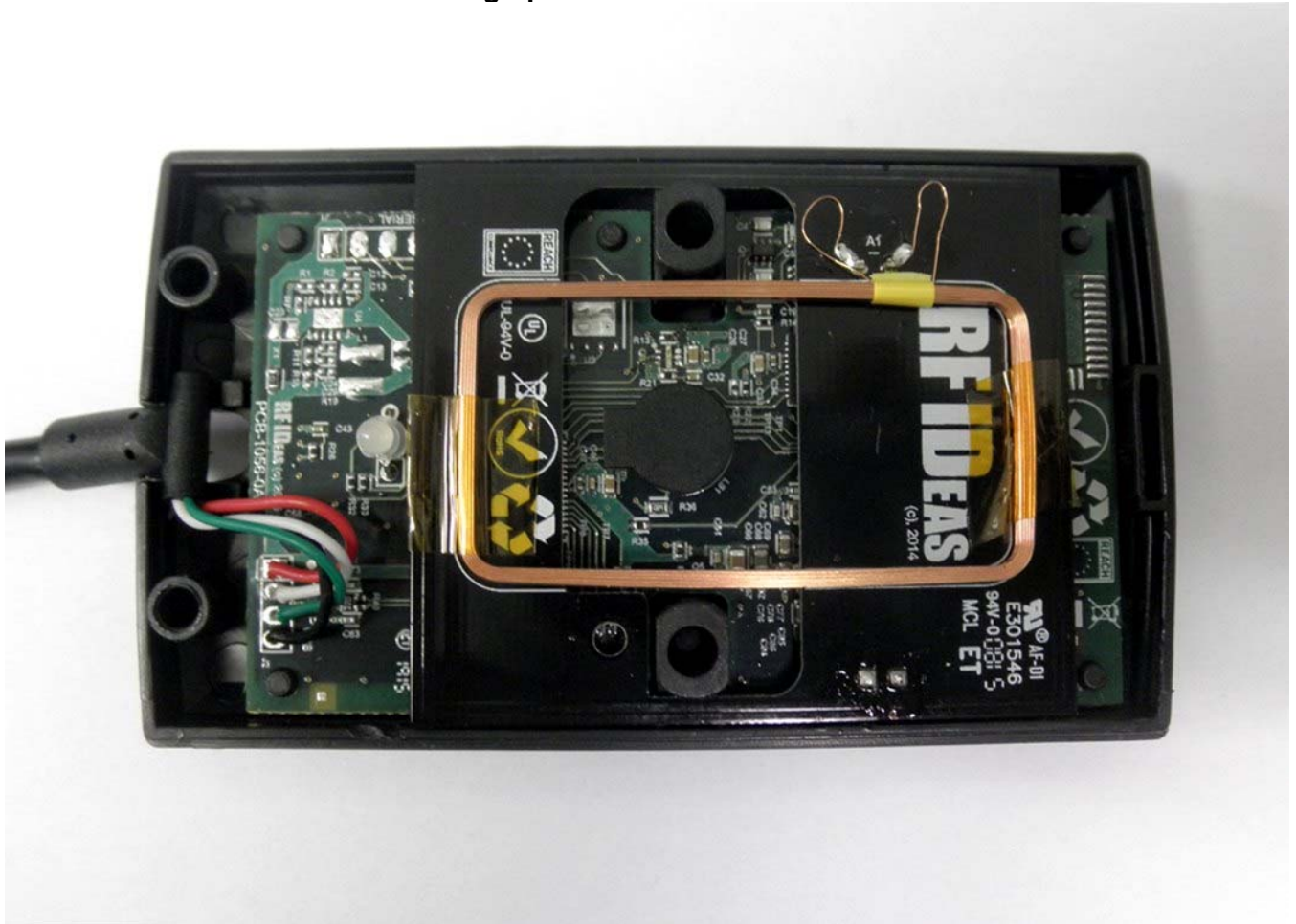
Photograph of EUT: Cover Removed
