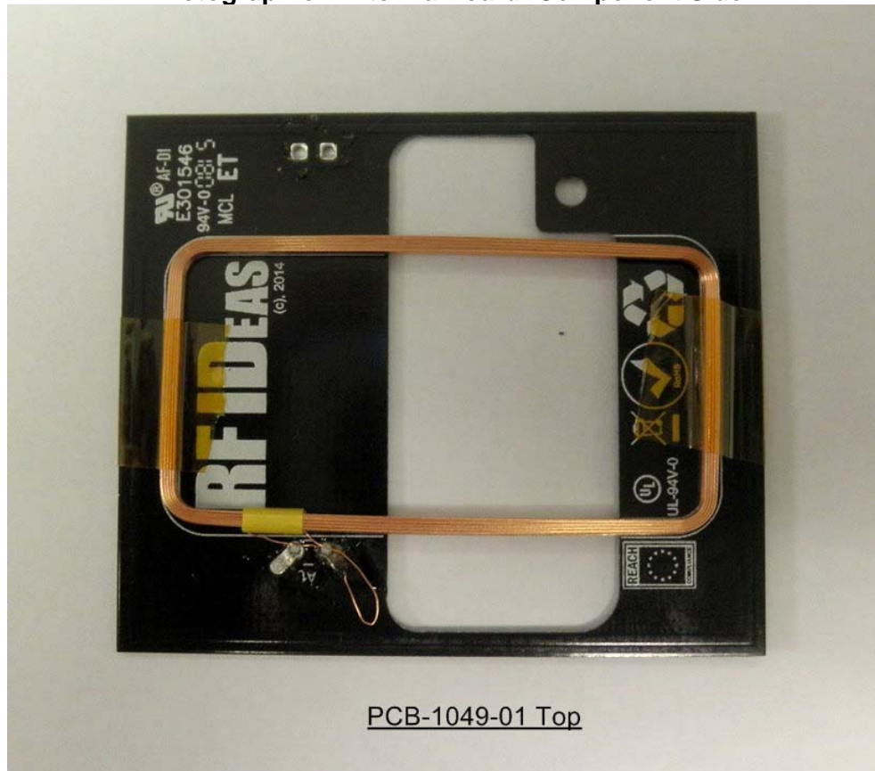
Photograph of Antenna Board: Foil Side
