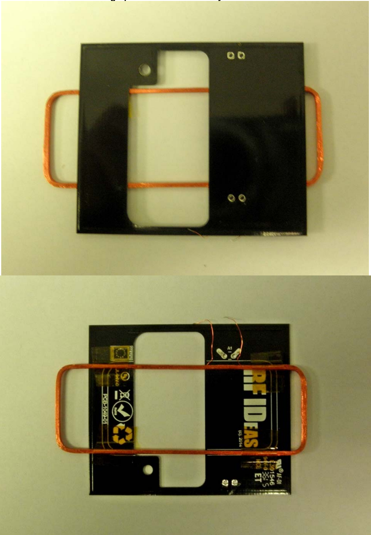
Photographs of Lower Assembly: Antenna Side
