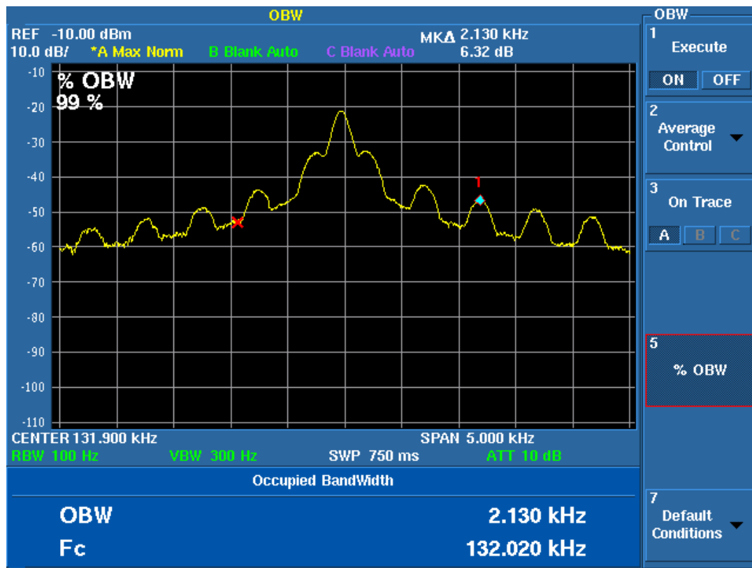
Figure 4. Occupied Bandwidth Plot: 132 kHz
