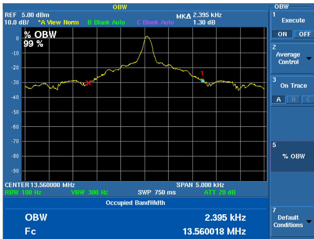
Figure 5. Occupied Bandwidth Plot: 13.56 MHz
