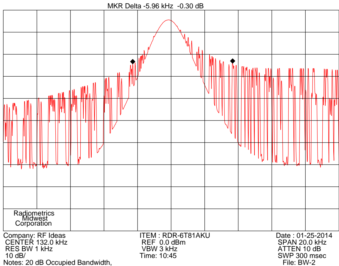
Figure 3. Occupied Bandwidth Plots 132 kHz
