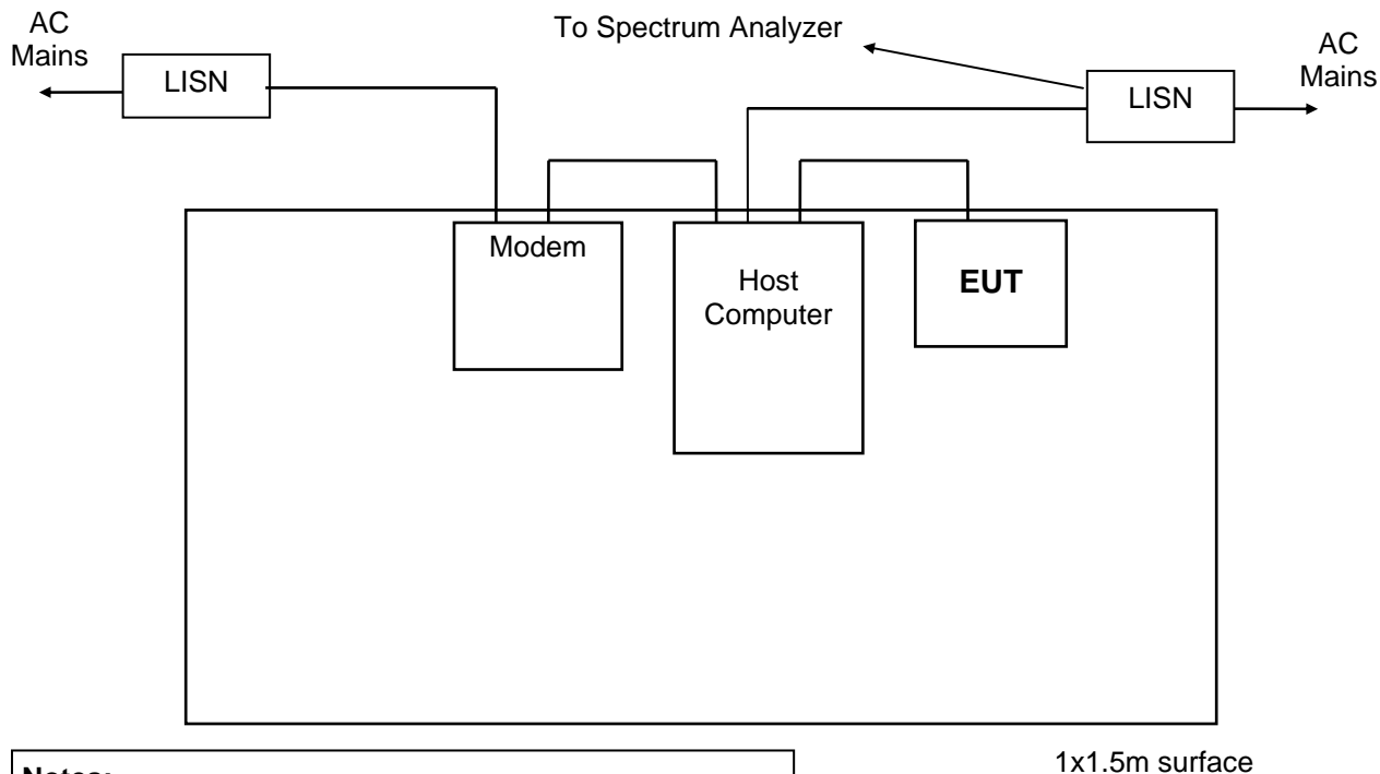
Figure 1. Conducted Emissions Test Setup (USB Reader)
