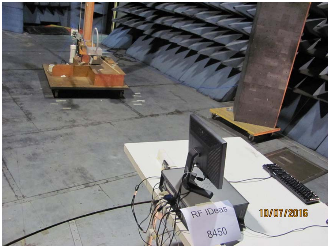
H-field 0.01-30 MHz
