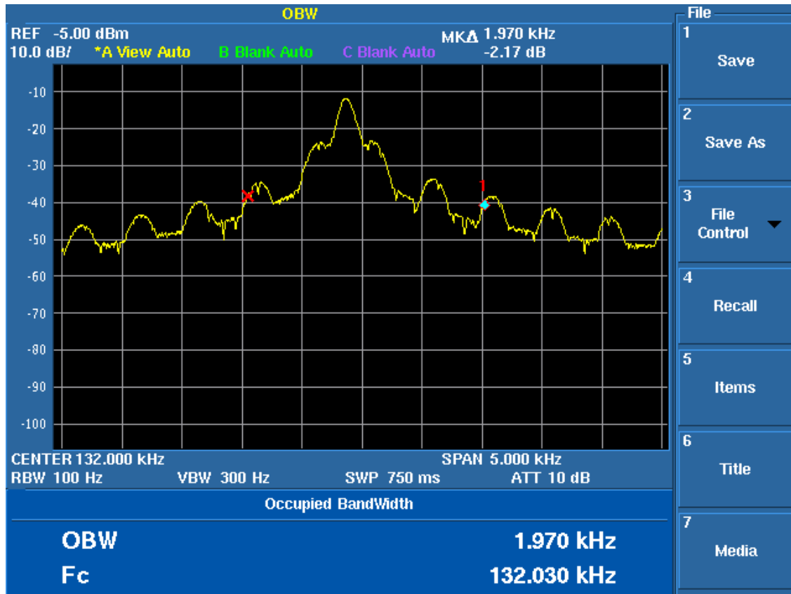
Figure 4. Occupied Bandwidth Plot: 132 kHz
