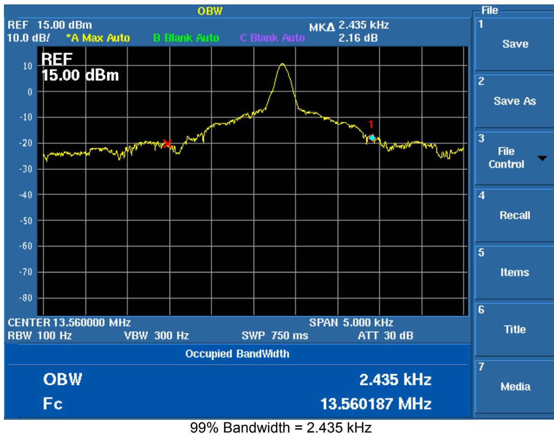
Figure 5. Occupied Bandwidth Plot: 13.56 MHz
