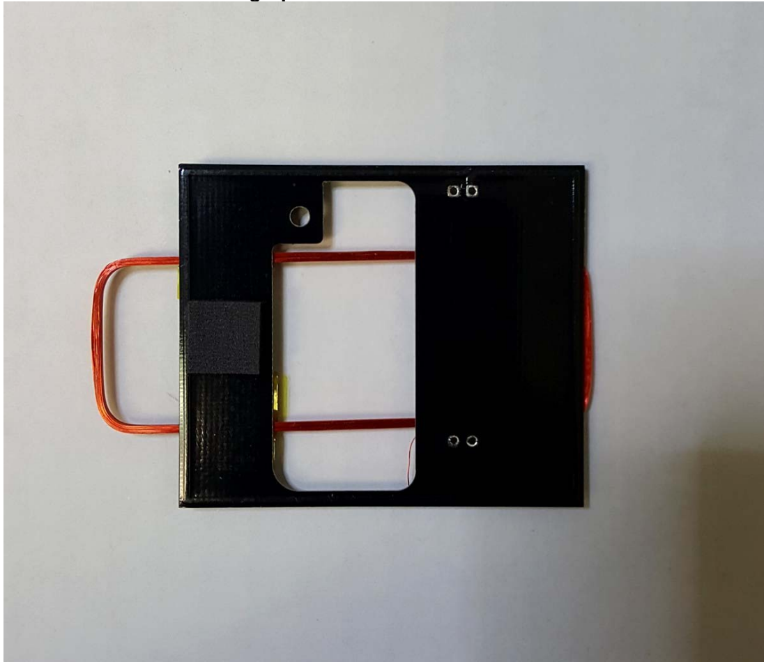
Photograph of Antenna Board: Foil side
