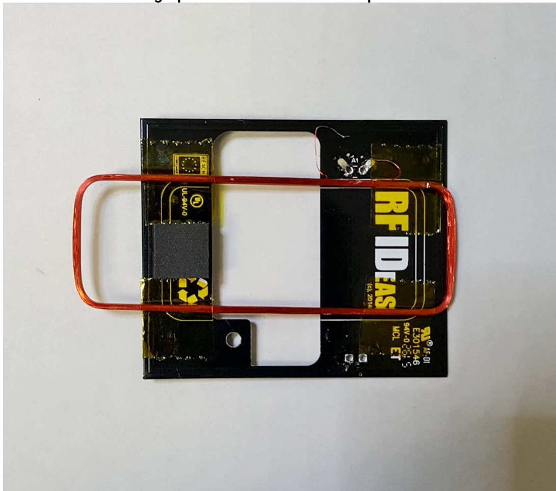
Photograph of Antenna Board: Component side
