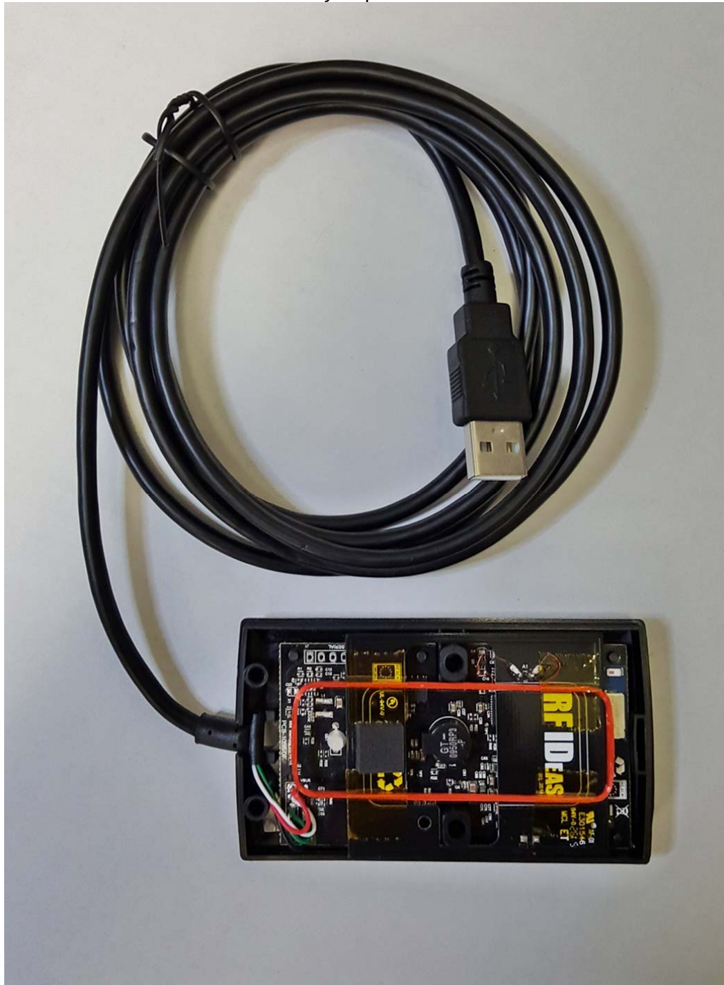
EUT Assembly-Top Cover Removed
