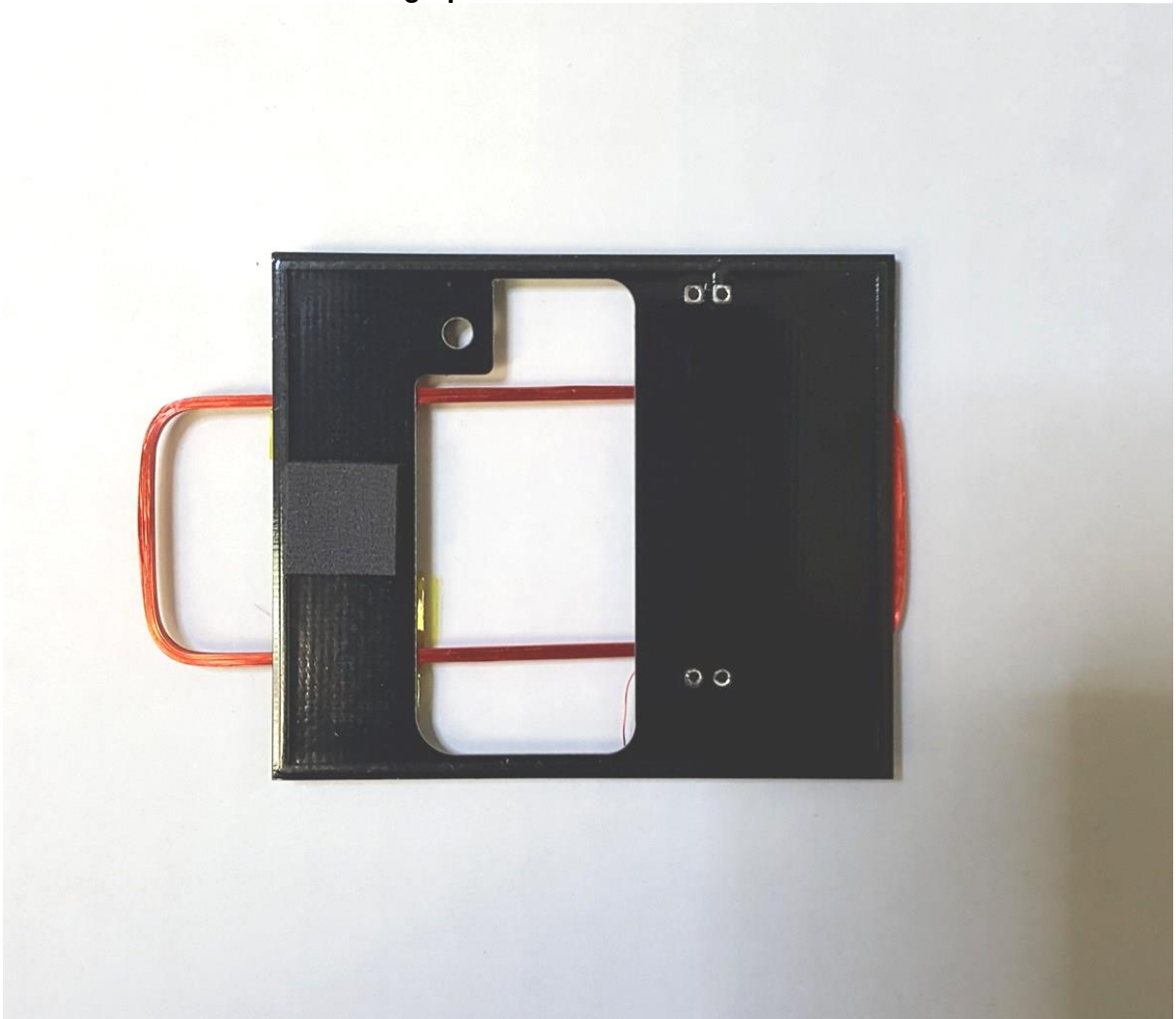
Photograph of Antenna Board: Foil side
