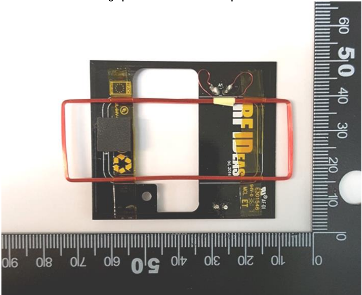
Photograph of Antenna Board: Component side
