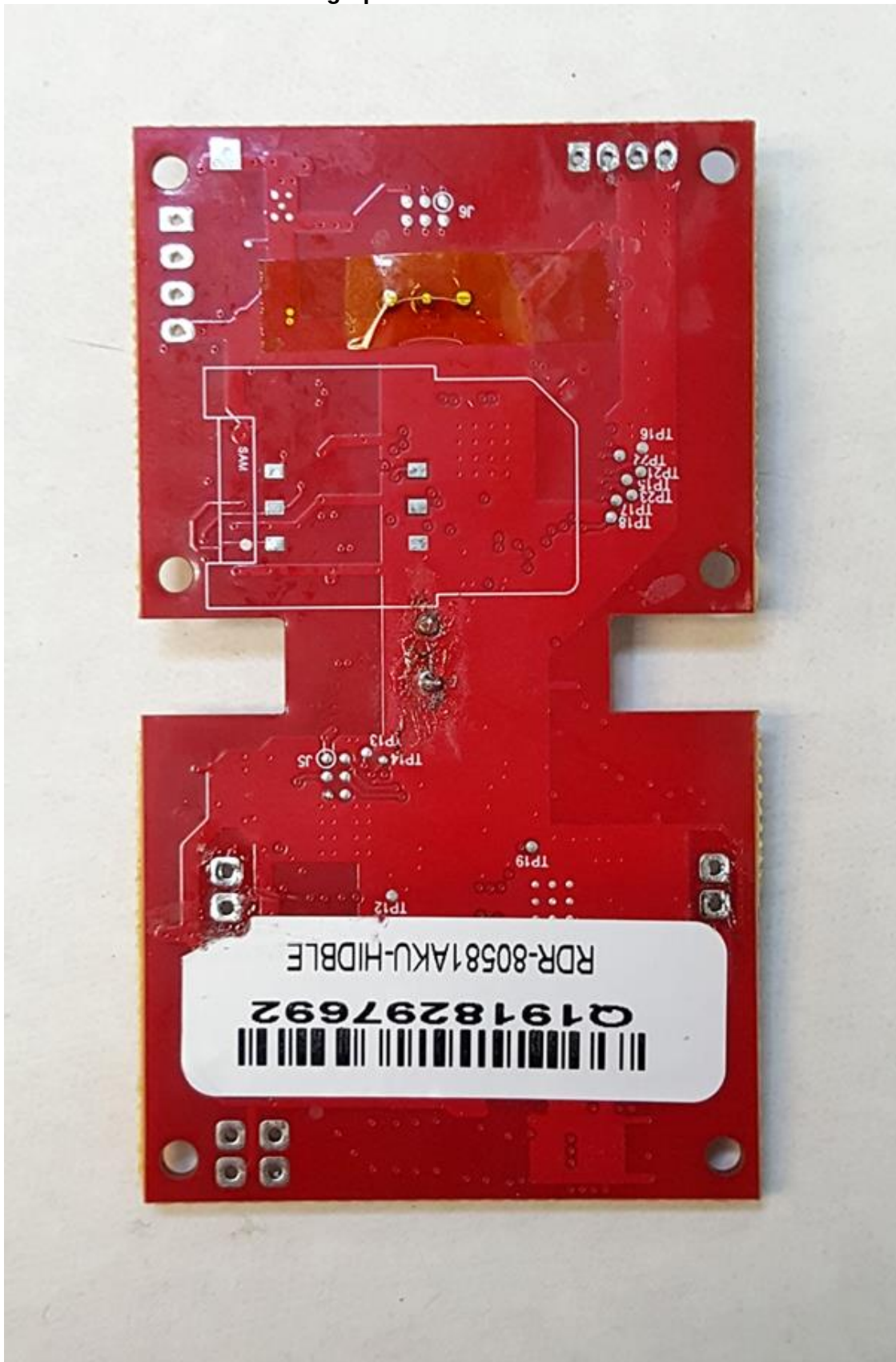
Photograph of PC Board: Foil Side
