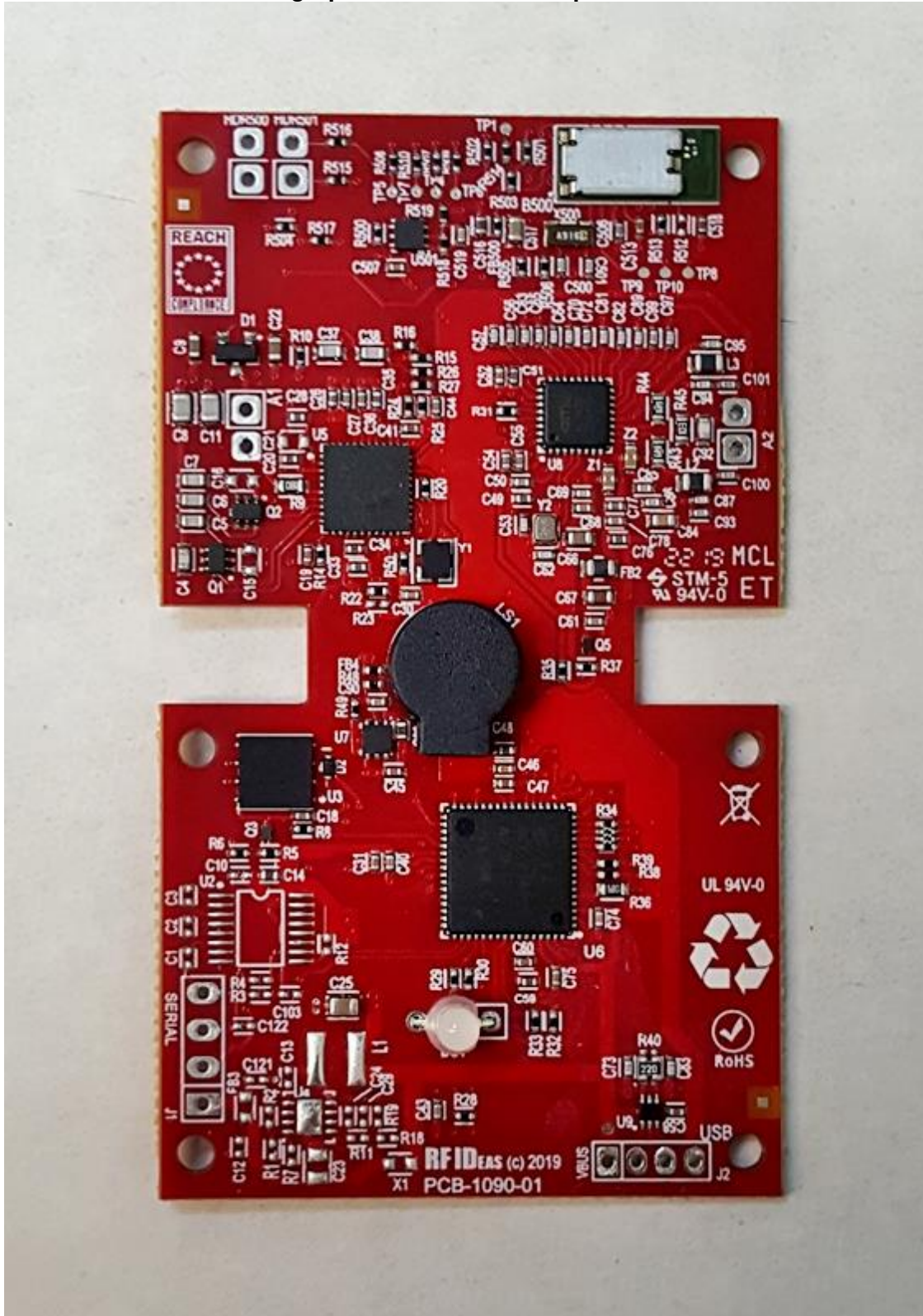
Photograph of PC Board: Component Side
