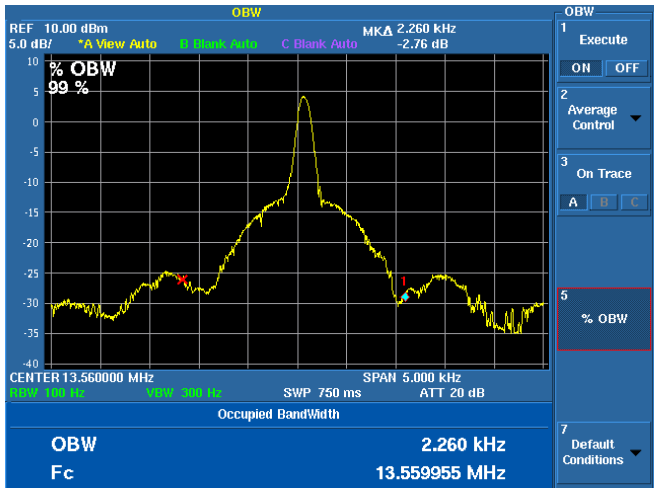
Figure 3. Occupied Bandwidth Plot 13.56 MHz
