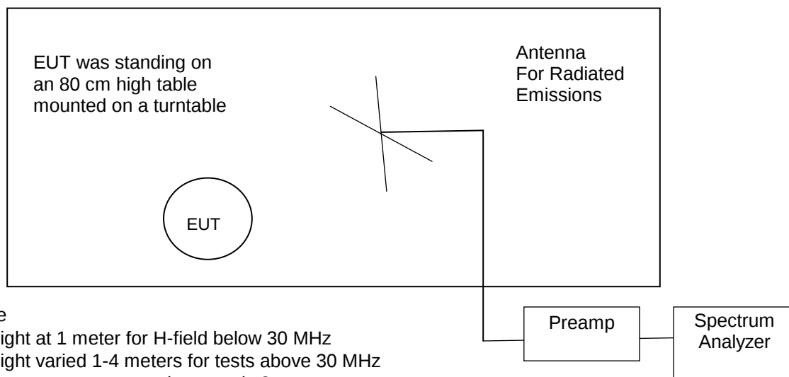
Figure 2. Drawing of Radiated Emissions Test Setup
