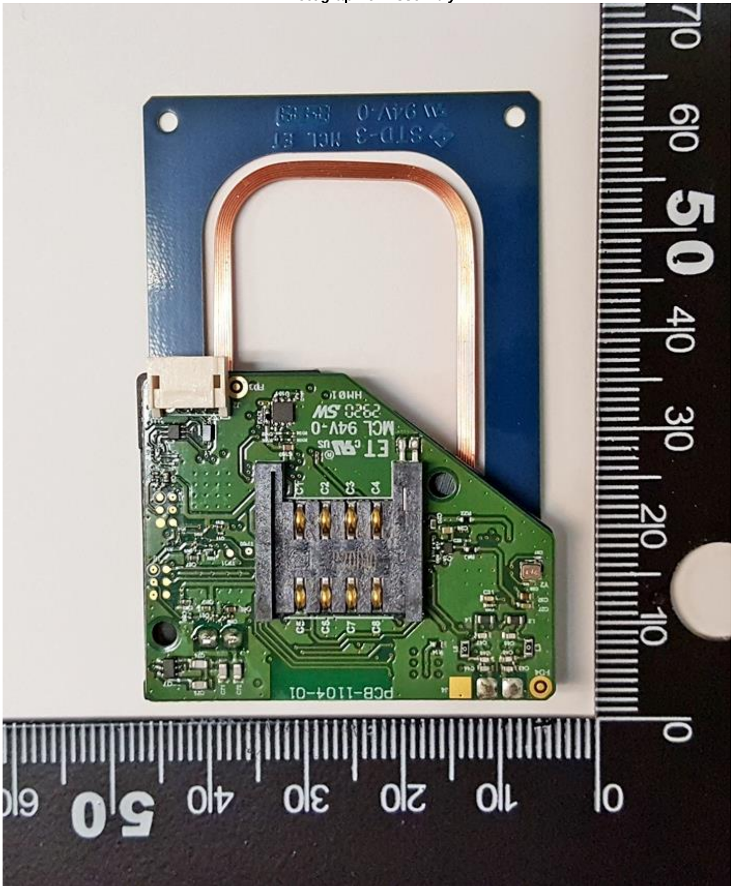
Photograph of Assembly
