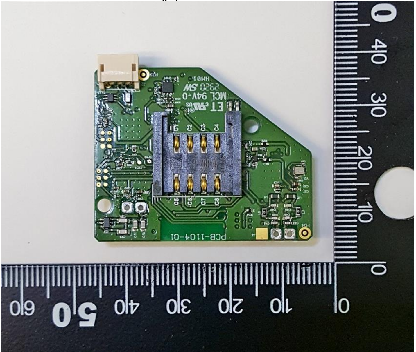
Photograph of PC Board: Foil Side
