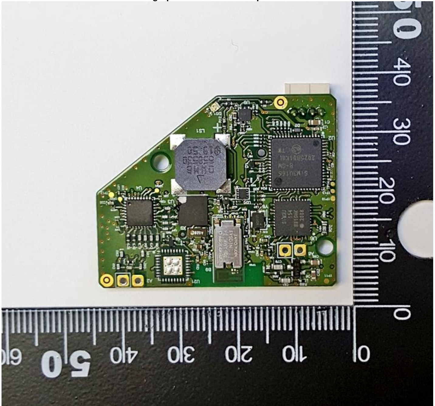
Photograph of PC Board: Component Side
