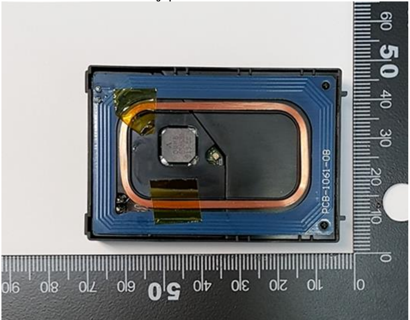
Photograph of EUT: Cover Removed
