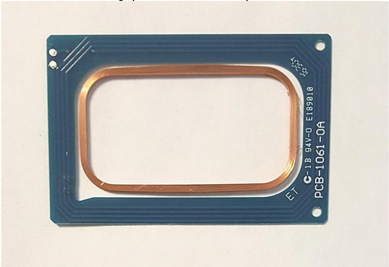
Photograph of Antenna Board: Foil Side
