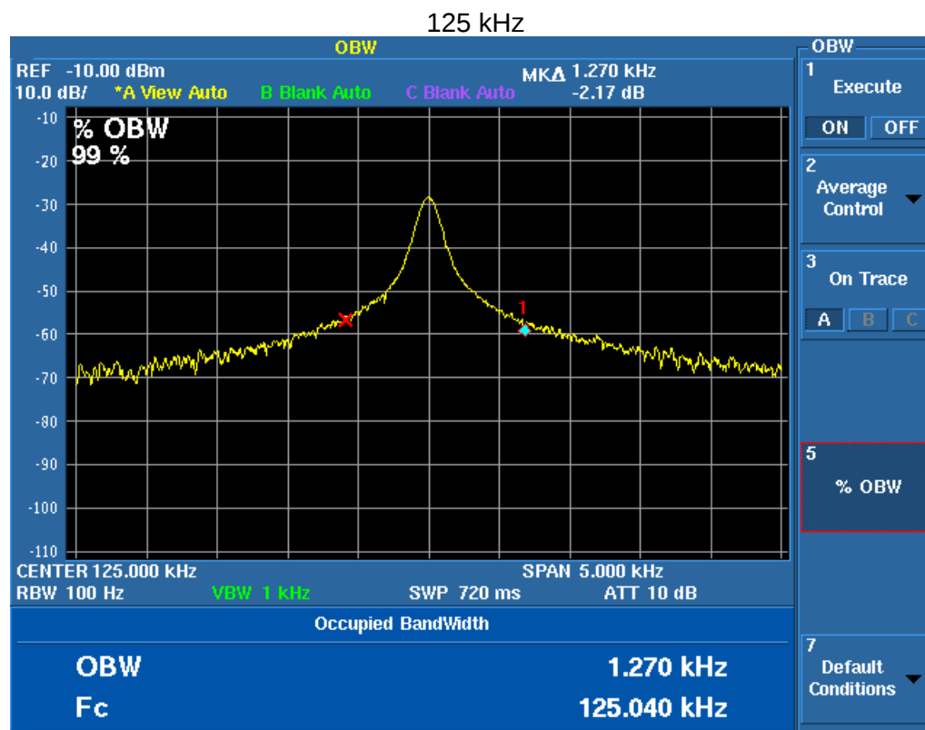
Figure 3. Occupied Bandwidth Plot
