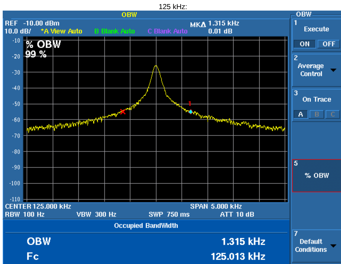
Figure 3. Occupied Bandwidth Plot
