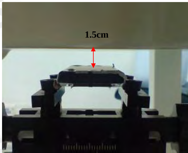
Fig.8 Body worn- EUT back to flat phantom and distance between flat phantom and mobile phone is 1.5 cm
