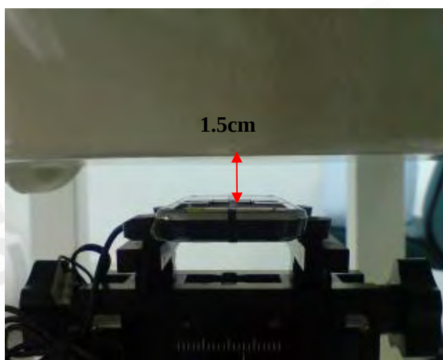
Fig.9 Body worn- EUT front to flat phantom and distance between flat phantom and mobile phone is 1.5 cm with headset
