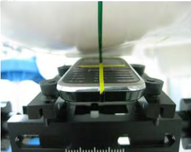
Fig.4 Right Head Ear-Tilt Position(15°)
