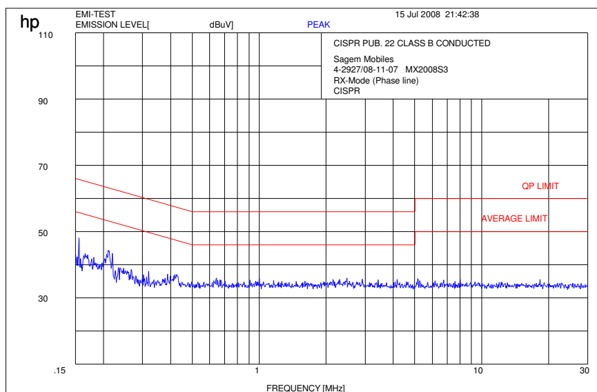
Plot 3: RX-Mode (Phase line)
