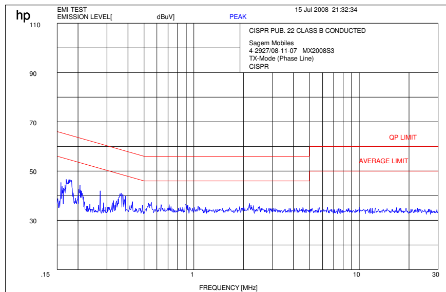
Plot 1: TX-Mode (Phase line)
