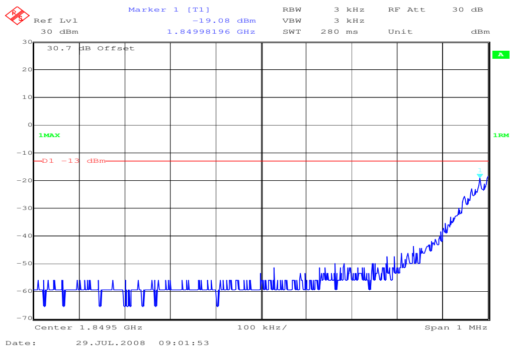
Plot 1: lower band edge (Channel 512)
