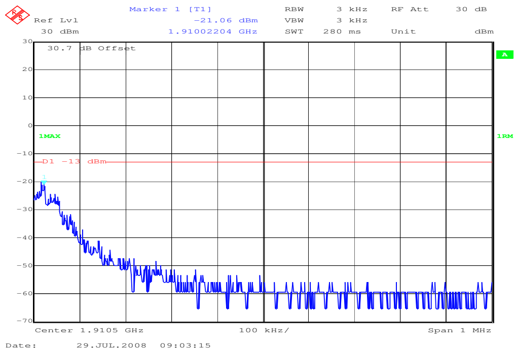
Plot 2: higher band edge (Channel 810)
