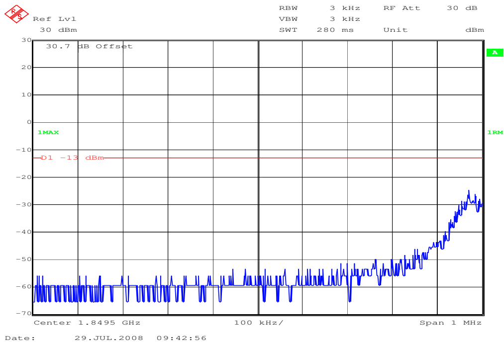
Plot 3: lower band edge (Channel 512 EDGE)
