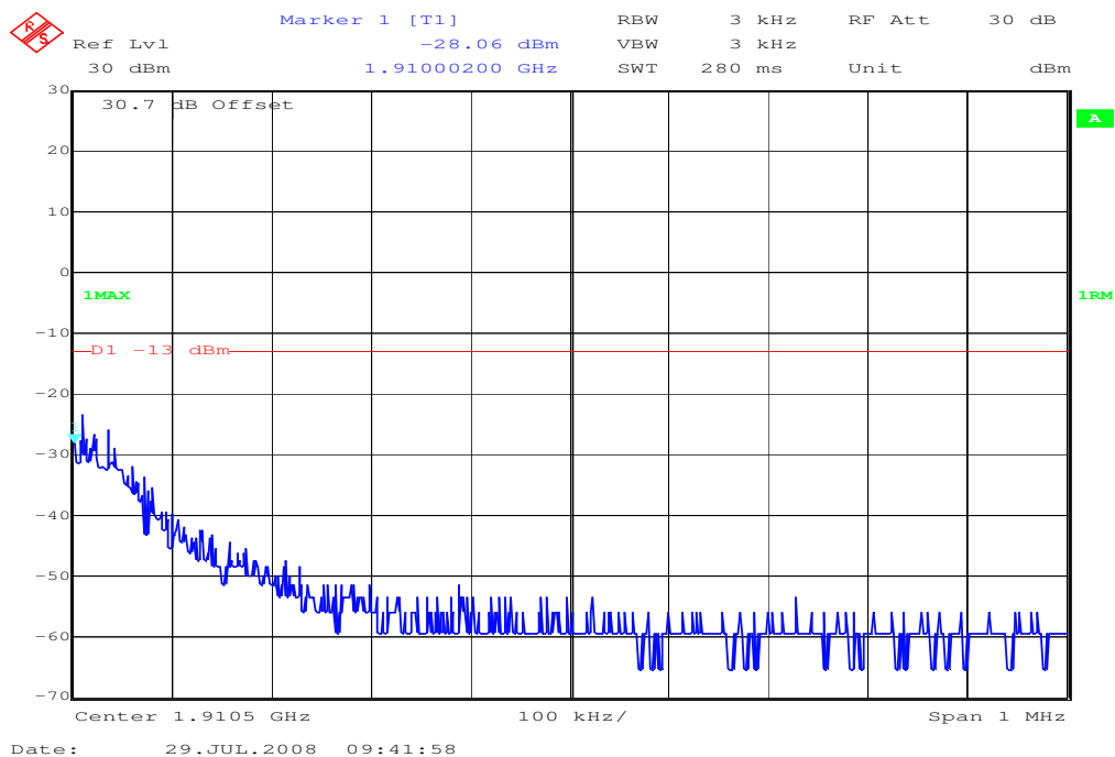
Plot 4: higher band edge (Channel 810 EDGE)
