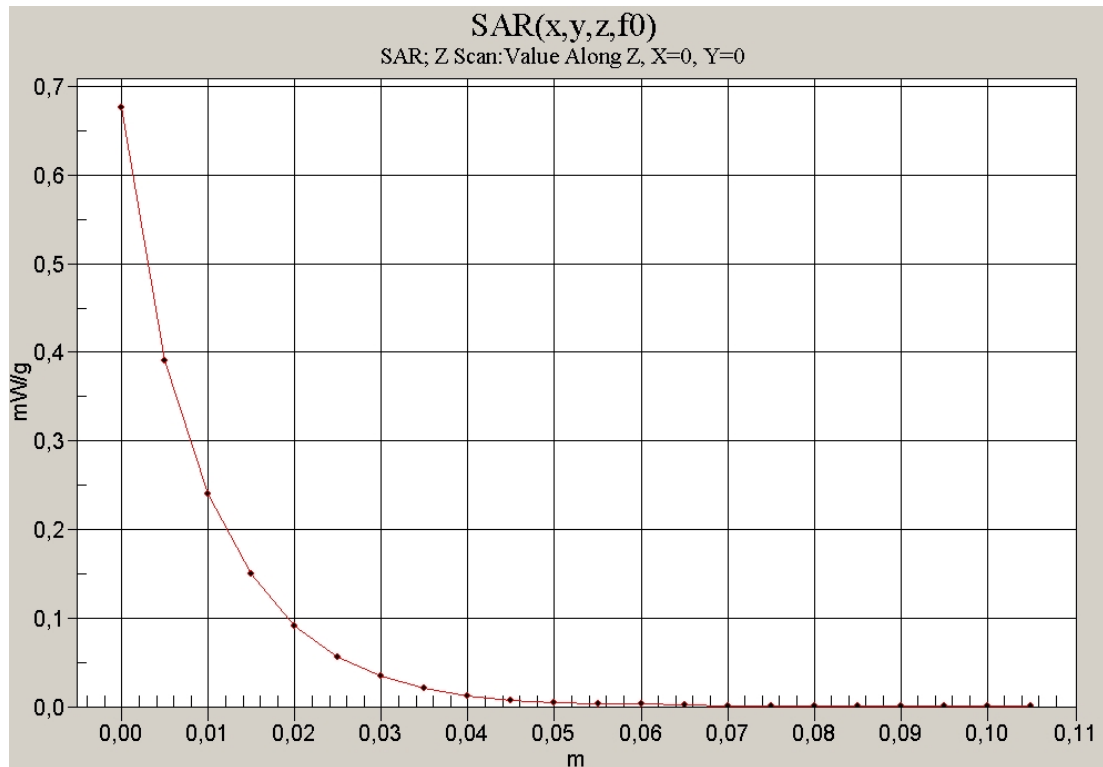
1900 MHz head with Bluetooth
