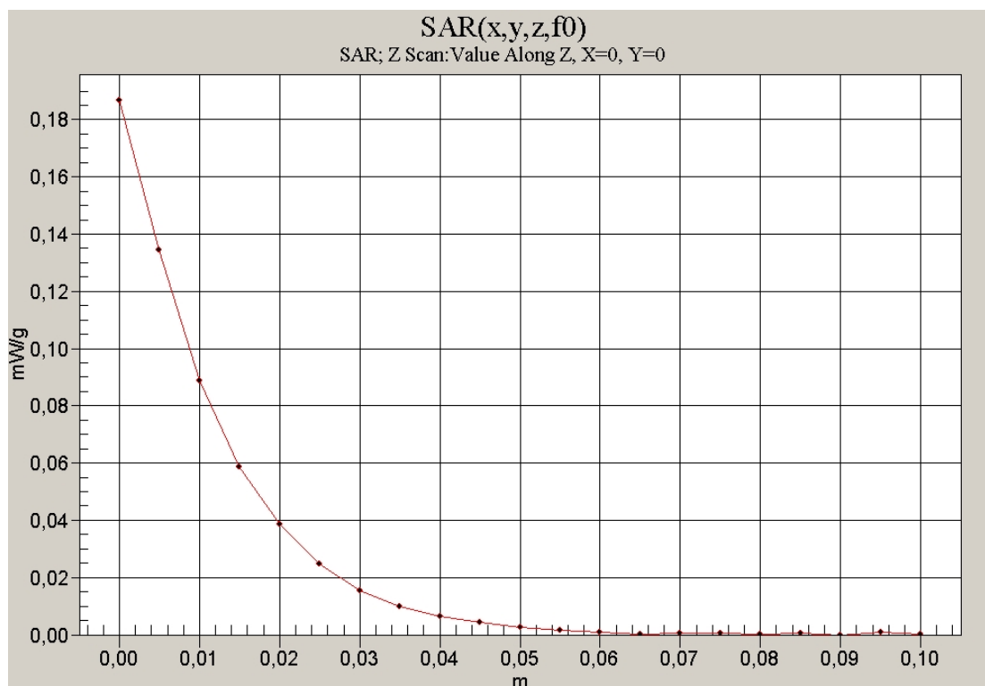
1900 MHz body with Bluetooth
