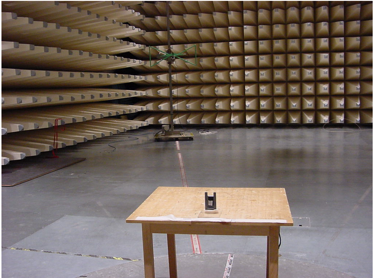
Photo 1: Radiated Emissions
