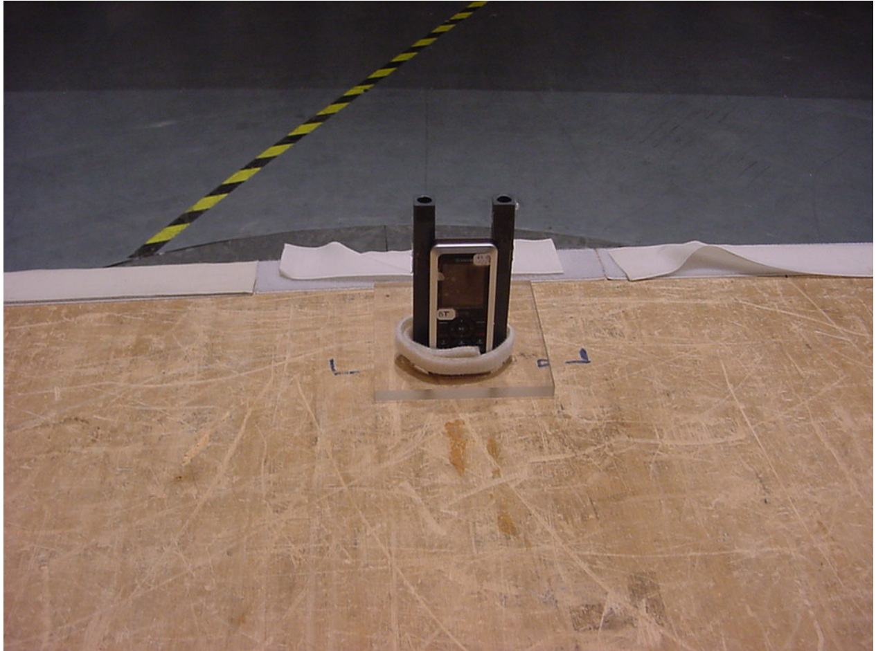
Photo 2: Radiated Emissions
