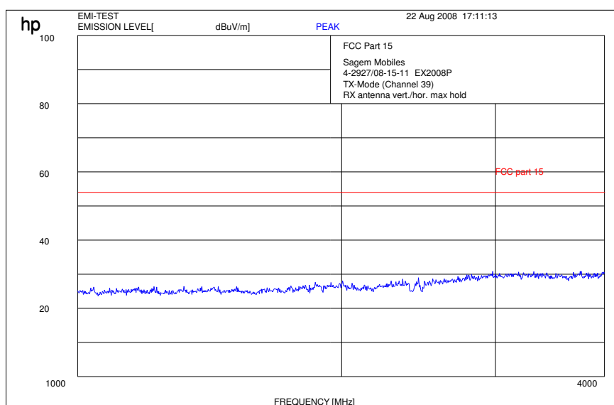
Plot 6: 1 - 4 GHz vertical/horizontal (middle channel)
