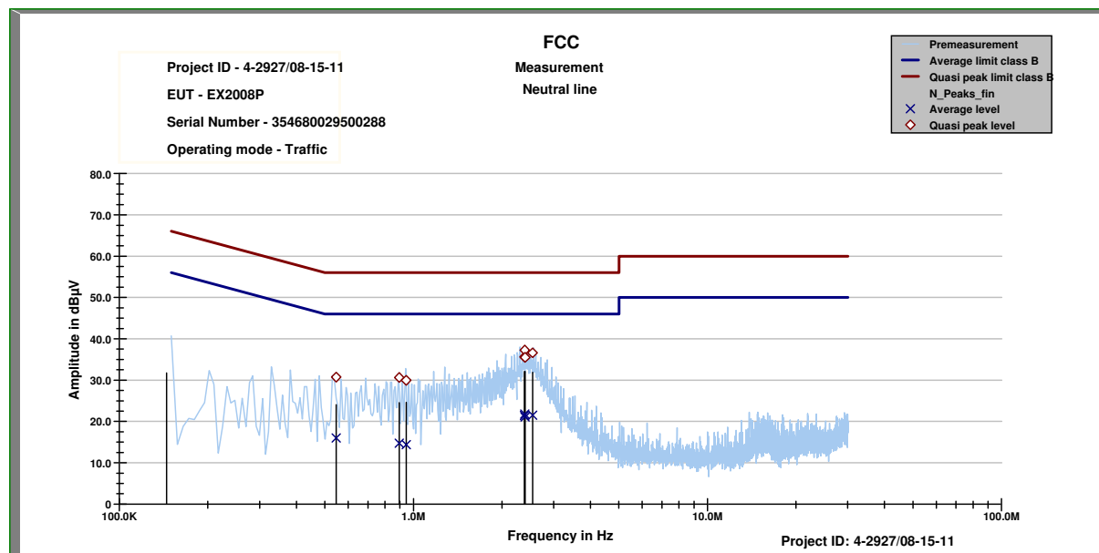
Plot 2: TX-Mode (Neutral Line)
