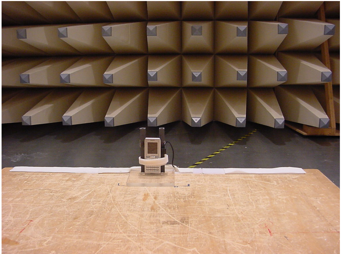
Photo 2: Radiated Emissions
