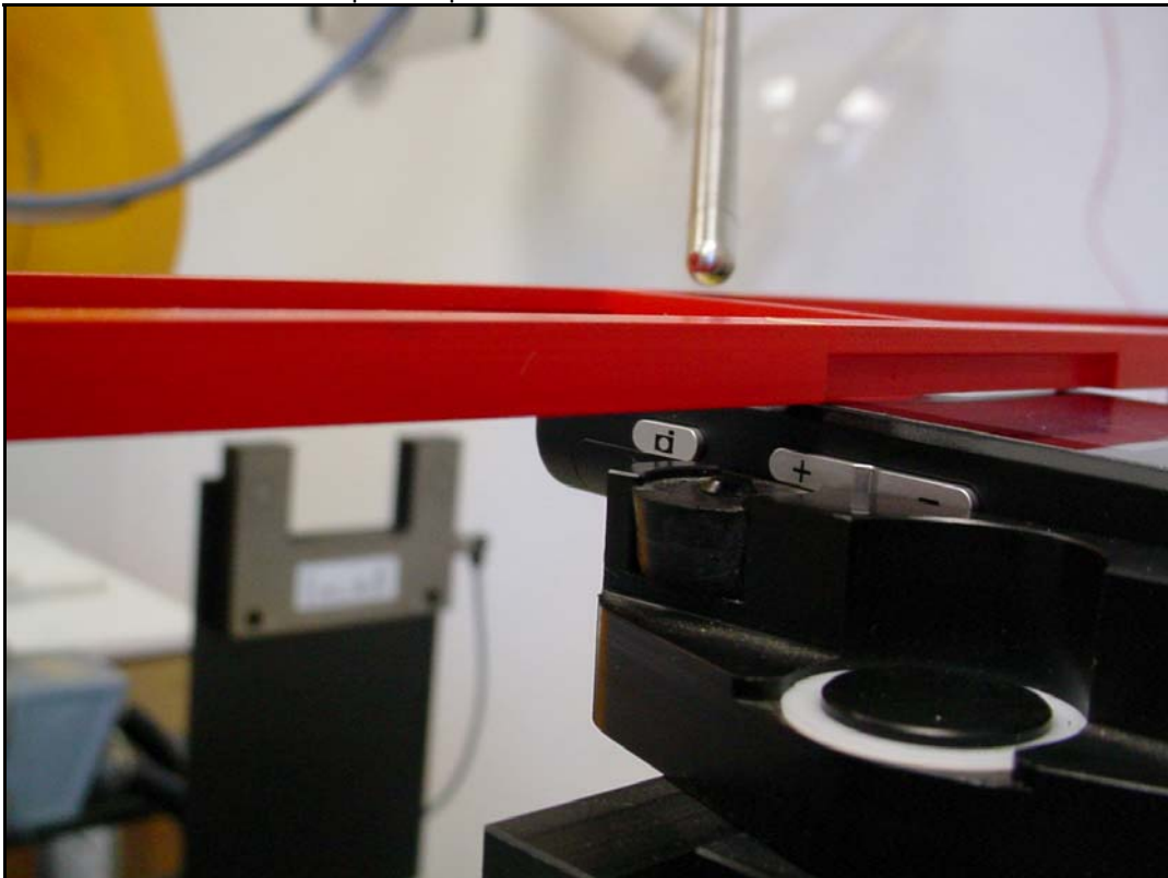
Photo 8: DUT at test position (side view)
