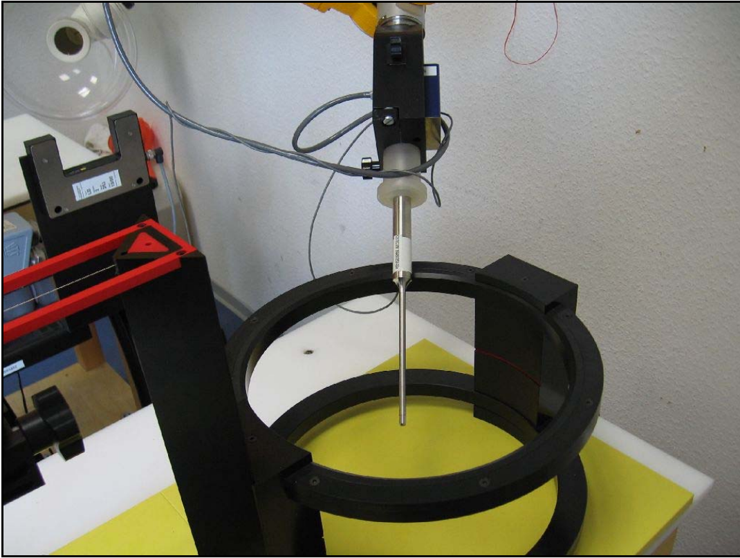
Photo 9: DUT - front view with HAC T-Coil position
