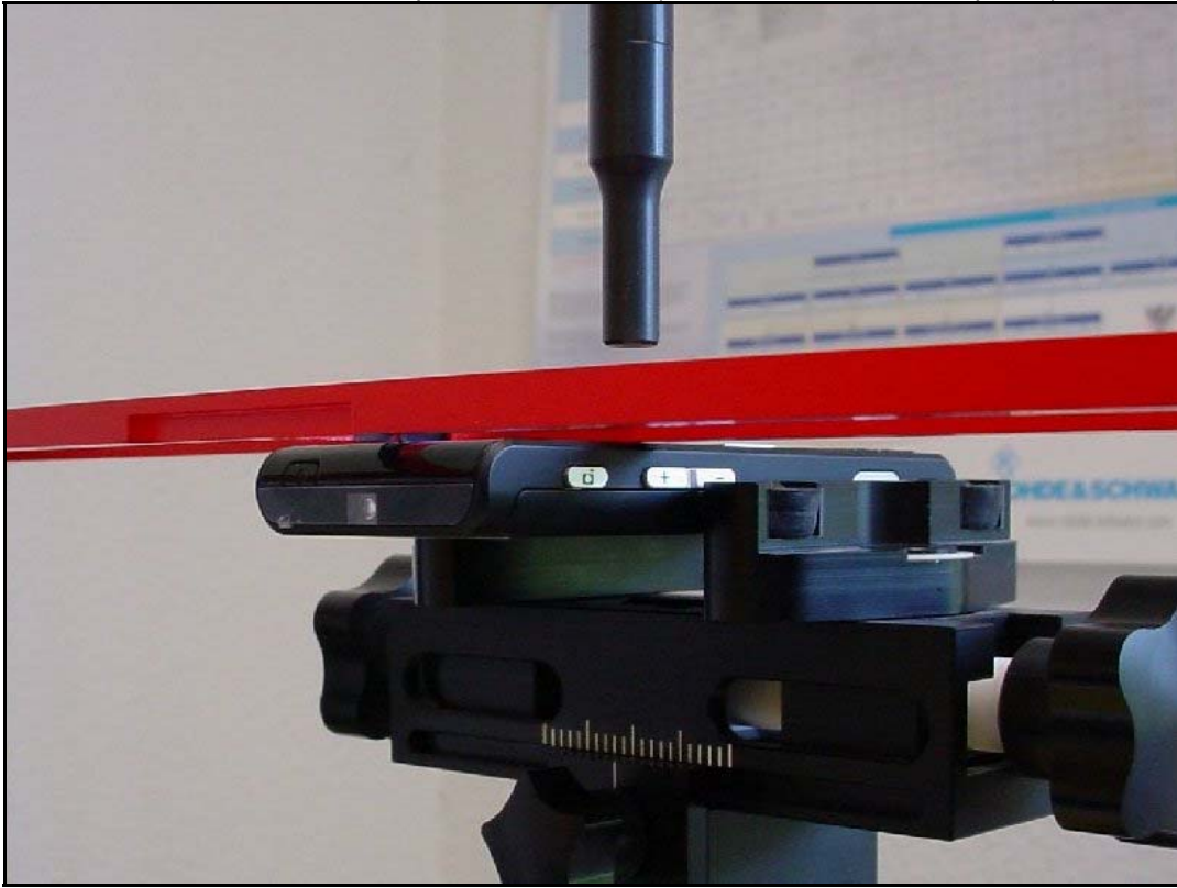
Photo 7: HAC RF test position with DUT (shown here with E-field probe)
