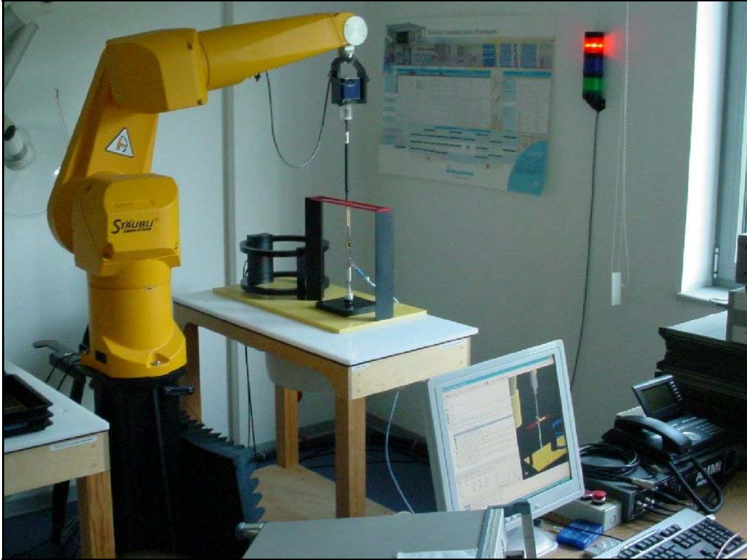
Photo 2: System validation (shown here with 1880 MHz dipole and H-field probe)
