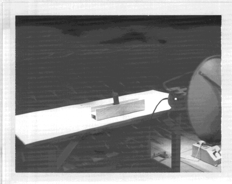
PCS mobile phone under test in anechoic chamber with the measurement antenna
