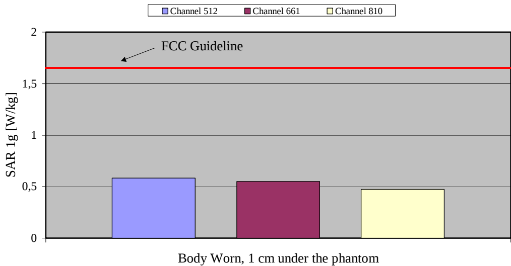
Fig. 8: The measured SAR values in body-worn configuration for the Sagem P52-6 for PCS 1900 in comparison to the FCC exposure limit.
