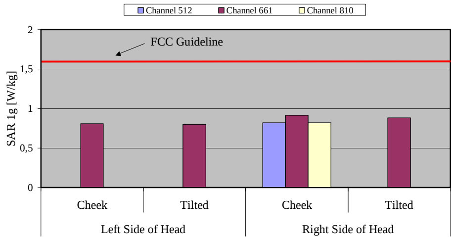
Fig. 7: The measured head phantom SAR values for the Sagem P52-6 for PCS 1900 in comparison to the FCC exposure limit.
